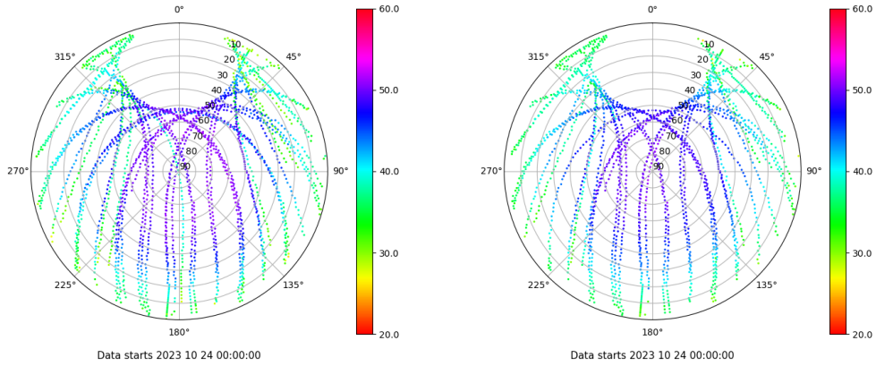
Skyplot for station SEV1. Signal to Noise S1C Data file SEV100ESP_R_2023297.xtr Skyplot for station SEV1. Signal to Noise S2C Data file SEV100ESP_R_2023297.xtr
