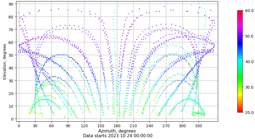
Azimuth-elevation plot for station SEV1. Signal to Noise S1C Data file SEV100ESP_R_2023297.xtr
