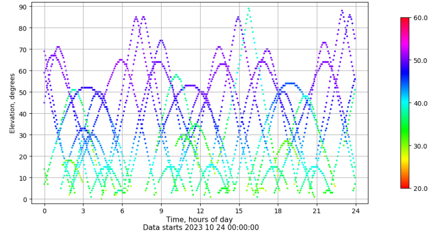
Time-elevation plot for station SEV1. Signal to Noise S1C Data file SEV100ESP_R_2023297.xtr
