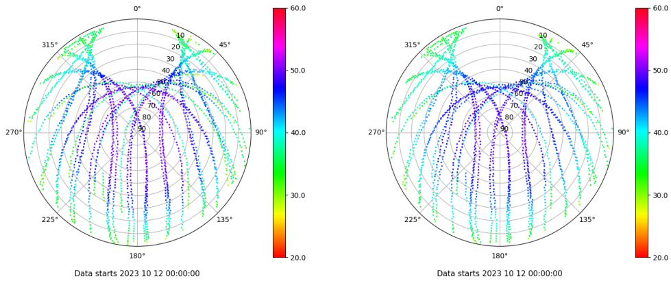
Skyplot for station SEV1. Signal to Noise S1C Data file SEV100ESP_R_2023285.xtr Skyplot for station SEV1. Signal to Noise S2C Data file SEV100ESP_R_2023285.xtr
