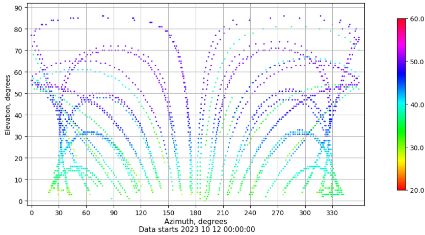
Azimuth-elevation plot for station SEV1. Signal to Noise S1C Data file SEV100ESP_R_2023285.xtr
