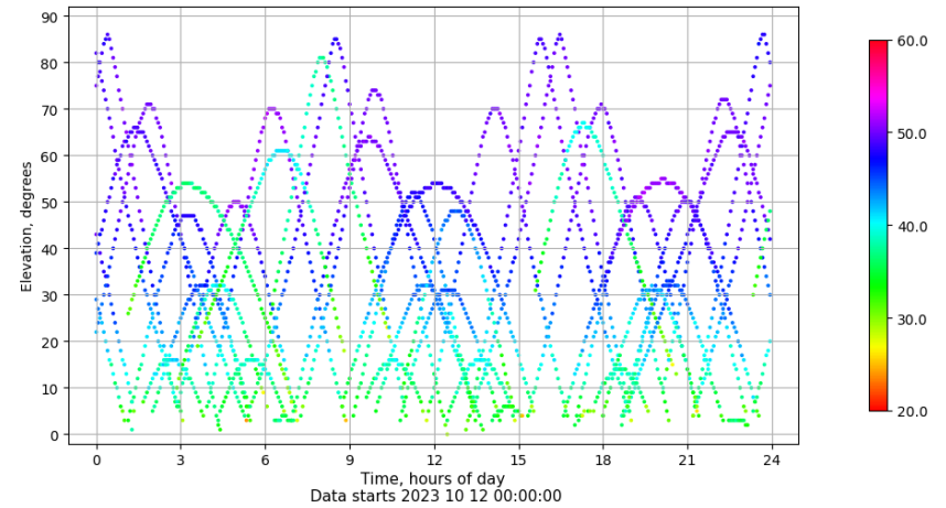
Time-elevation plot for station SEV1. Signal to Noise S1C Data file SEV100ESP_R_2023285.xtr
