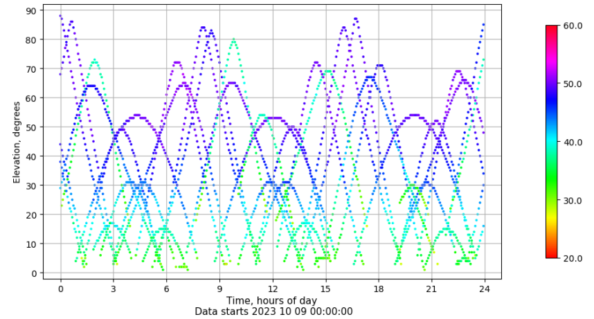
Time-elevation plot for station SEV1. Signal to Noise S1C Data file SEV100ESP_R_2023282.xtr
