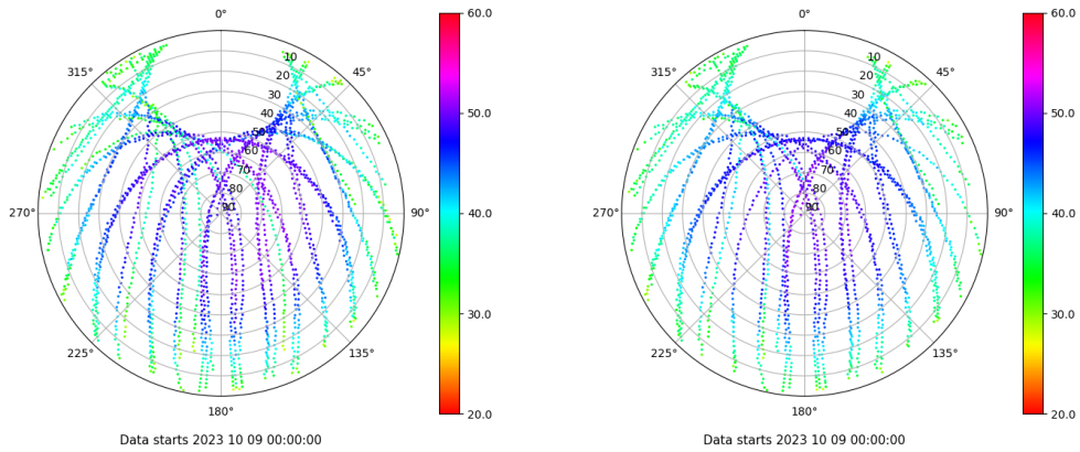
Skyplot for station SEV1. Signal to Noise S1C Data file SEV100ESP_R_2023282.xtr Skyplot for station SEV1. Signal to Noise S2C Data file SEV100ESP_R_2023282.xtr
