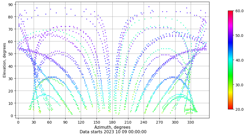
Azimuth-elevation plot for station SEV1. Signal to Noise S1C Data file SEV100ESP_R_2023282.xtr
