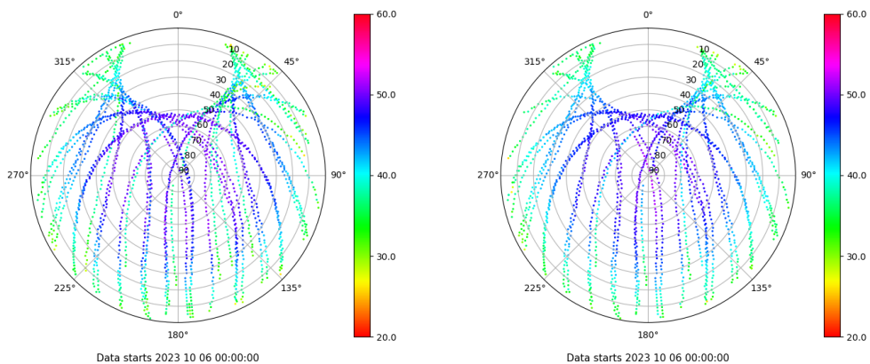
Skyplot for station SEV1. Signal to Noise S1C Data file SEV100ESP_R_2023279.xtr Skyplot for station SEV1. Signal to Noise S2C Data file SEV100ESP_R_2023279.xtr
