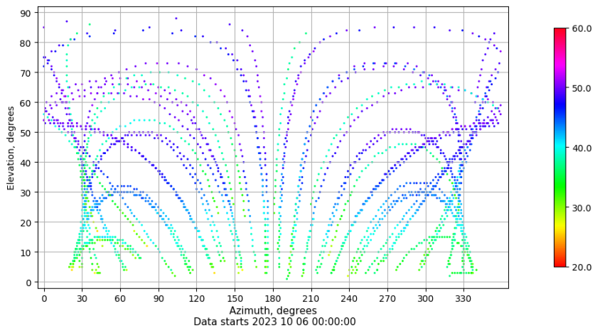
Azimuth-elevation plot for station SEV1. Signal to Noise S1C Data file SEV100ESP_R_2023279.xtr
