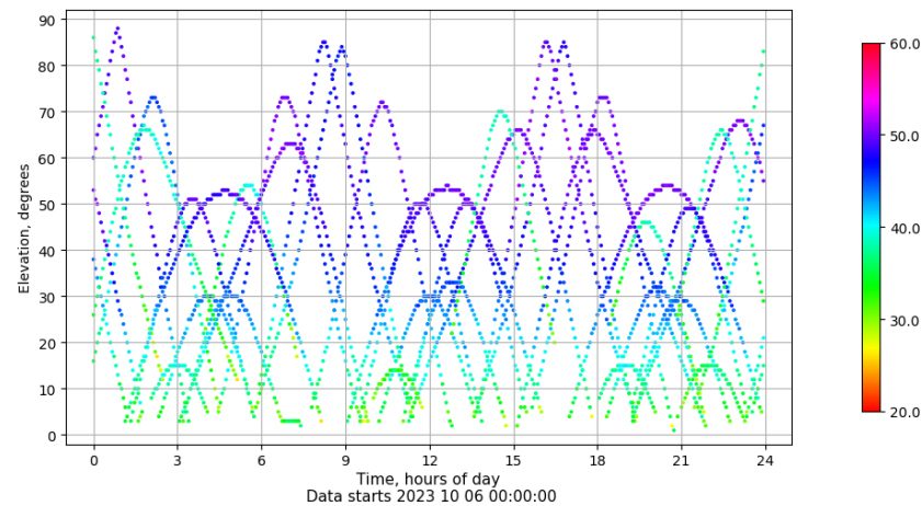
Time-elevation plot for station SEV1. Signal to Noise S1C Data file SEV100ESP_R_2023279.xtr
