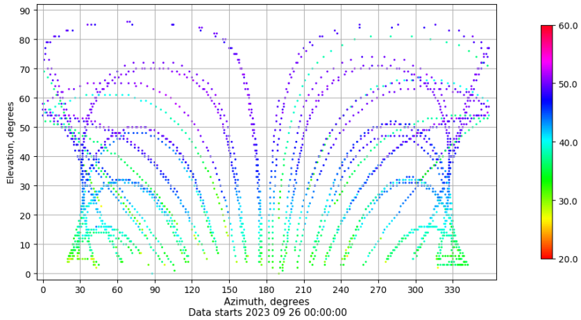
Azimuth-elevation plot for station SEV1. Signal to Noise S1C Data file SEV100ESP_R_2023269.xtr
