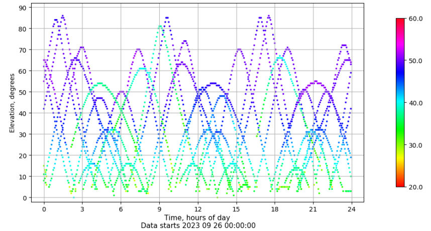
Time-elevation plot for station SEV1. Signal to Noise S1C Data file SEV100ESP_R_2023269.xtr
