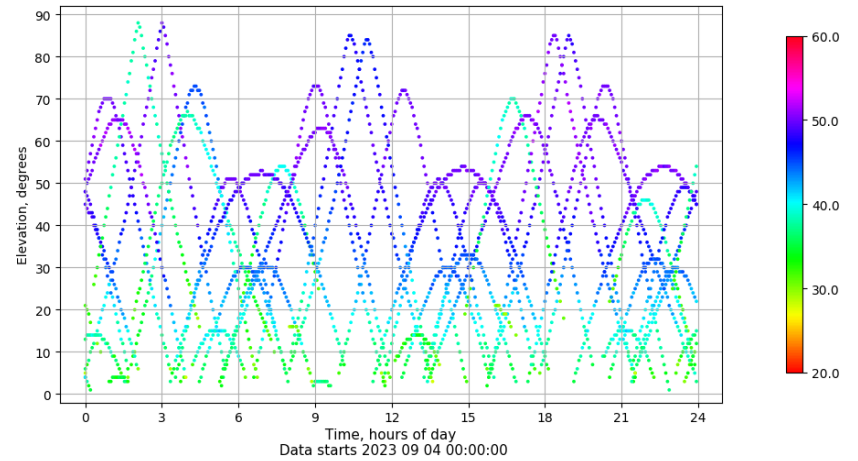
Time-elevation plot for station SEV1. Signal to Noise S1C Data file SEV100ESP_R_2023247.xtr
