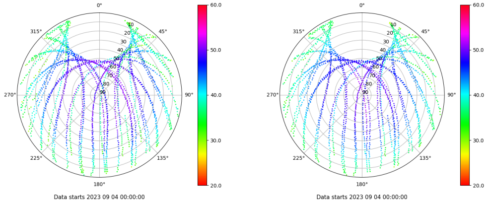
Skyplot for station SEV1. Signal to Noise S1C Data file SEV100ESP_R_2023247.xtr Skyplot for station SEV1. Signal to Noise S2C Data file SEV100ESP_R_2023247.xtr
