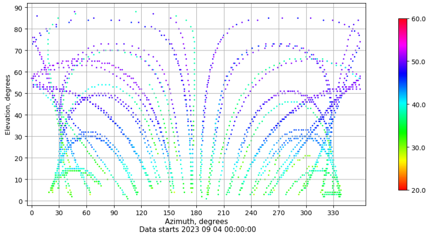
Azimuth-elevation plot for station SEV1. Signal to Noise S1C Data file SEV100ESP_R_2023247.xtr
