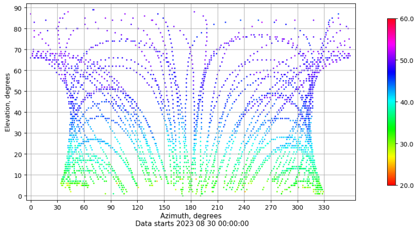
Azimuth-elevation plot for station SEV1. Signal to Noise S1C Data file SEV100ESP_R_2023242.xtr
