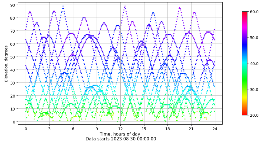
Time-elevation plot for station SEV1. Signal to Noise S1C Data file SEV100ESP_R_2023242.xtr
