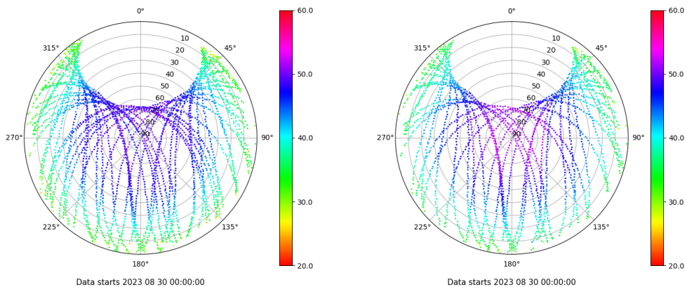
Skyplot for station SEV1. Signal to Noise S1C Data file SEV100ESP_R_2023242.xtr Skyplot for station SEV1. Signal to Noise S2X Data file SEV100ESP_R_2023242.xtr
