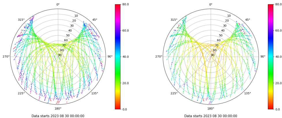
Skyplot for station SEV1. Parameter M1C Data file SEV100ESP_R_2023242.xtr Skyplot for station SEV1. Parameter M2X Data file SEV100ESP_R_2023242.xtr
