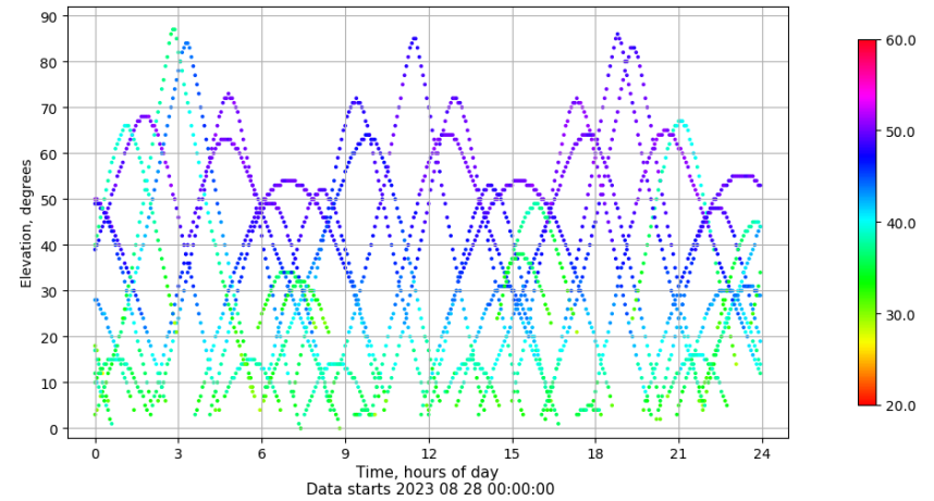
Time-elevation plot for station SEV1. Signal to Noise S1C Data file SEV100ESP_R_2023240.xtr
