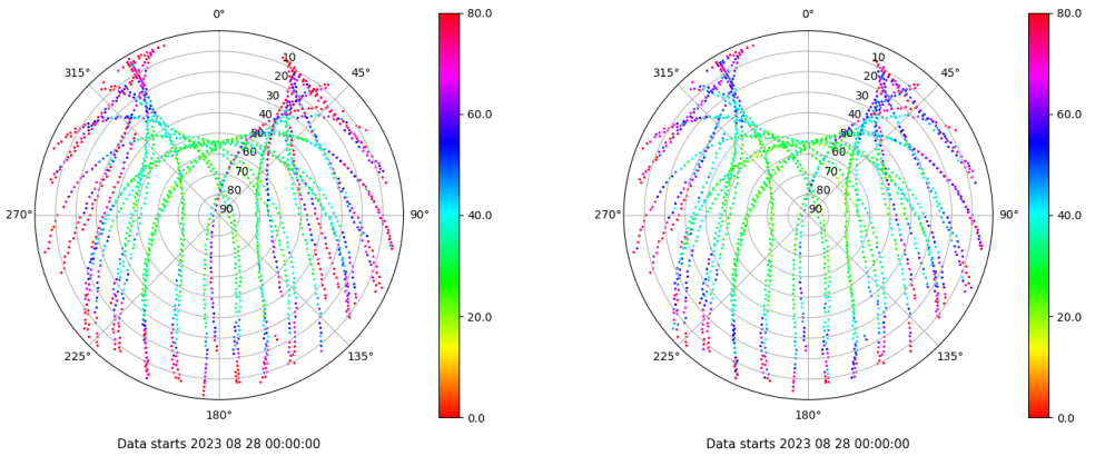
Skyplot for station SEV1. Parameter M1C Data file SEV100ESP_R_2023240.xtr Skyplot for station SEV1. Parameter M2C Data file SEV100ESP_R_2023240.xtr
