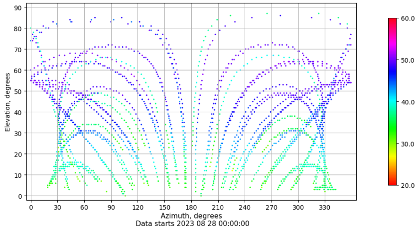
Azimuth-elevation plot for station SEV1. Signal to Noise S1C Data file SEV100ESP_R_2023240.xtr
