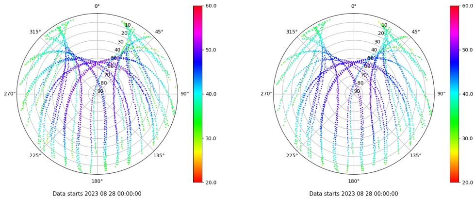
Skyplot for station SEV1. Signal to Noise S1C Data file SEV100ESP_R_2023240.xtr Skyplot for station SEV1. Signal to Noise S2C Data file SEV100ESP_R_2023240.xtr
