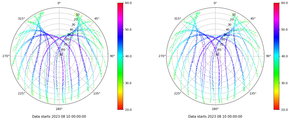
Skyplot for station SEV1. Signal to Noise S1C Data file SEV100ESP_R_2023222.xtr Skyplot for station SEV1. Signal to Noise S2C Data file SEV100ESP_R_2023222.xtr
