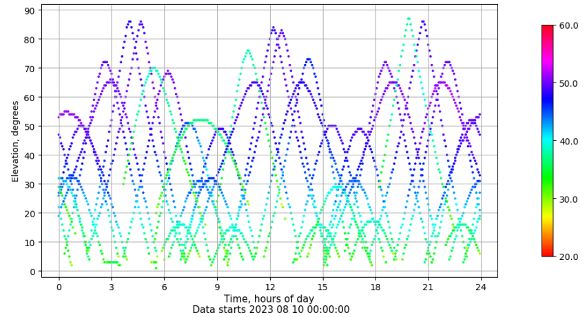
Time-elevation plot for station SEV1. Signal to Noise S1C Data file SEV100ESP_R_2023222.xtr
