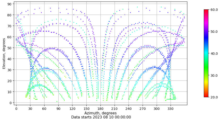
Azimuth-elevation plot for station SEV1. Signal to Noise S1C Data file SEV100ESP_R_2023222.xtr
