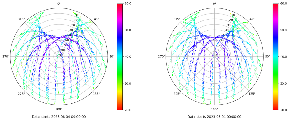
Skyplot for station SEV1. Signal to Noise S1C Data file SEV100ESP_R_2023216.xtr Skyplot for station SEV1. Signal to Noise S2C Data file SEV100ESP_R_2023216.xtr
