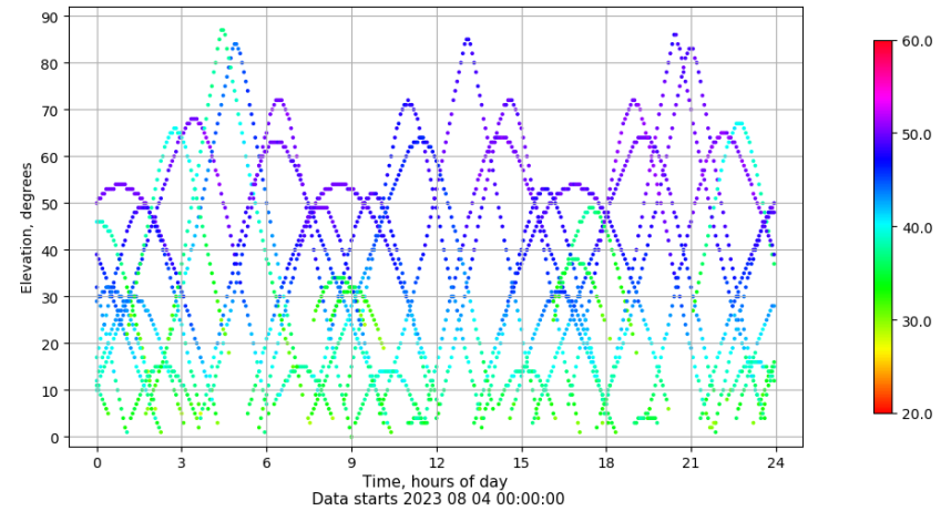
Time-elevation plot for station SEV1. Signal to Noise S1C Data file SEV100ESP_R_2023216.xtr
