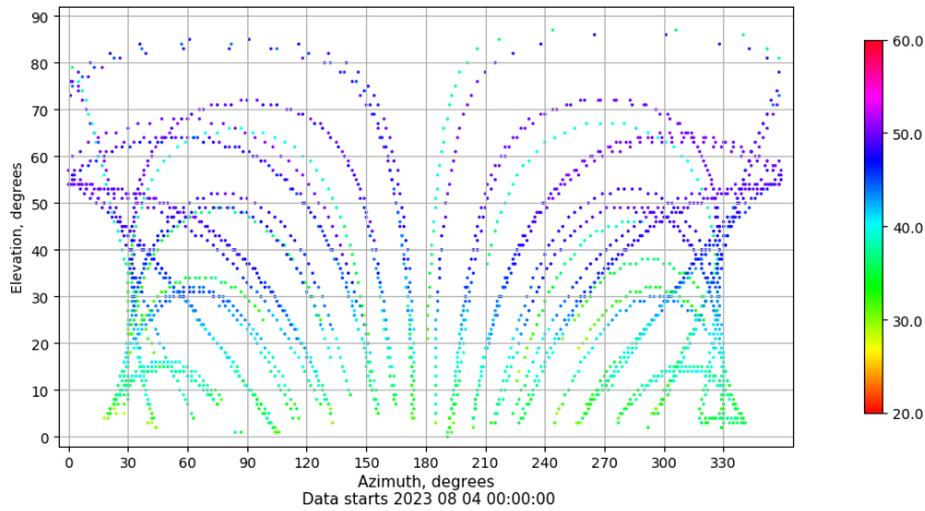
Azimuth-elevation plot for station SEV1. Signal to Noise S1C Data file SEV100ESP_R_2023216.xtr
