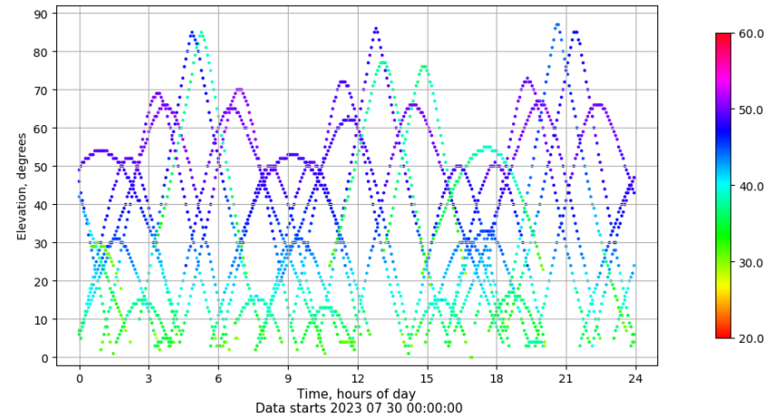
Time-elevation plot for station SEV1. Signal to Noise S1C Data file SEV100ESP_R_2023211.xtr
