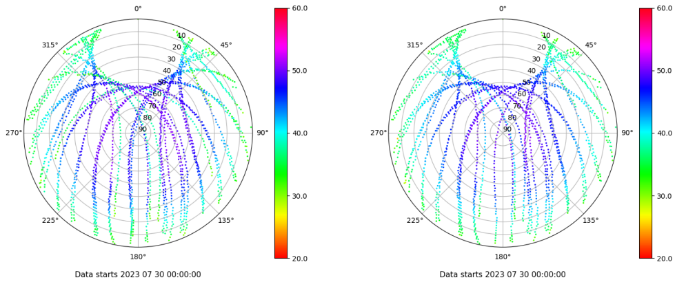
Skyplot for station SEV1. Signal to Noise S1C Data file SEV100ESP_R_2023211.xtr Skyplot for station SEV1. Signal to Noise S2C Data file SEV100ESP_R_2023211.xtr
