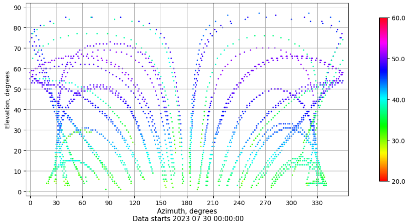
Azimuth-elevation plot for station SEV1. Signal to Noise S1C Data file SEV100ESP_R_2023211.xtr
