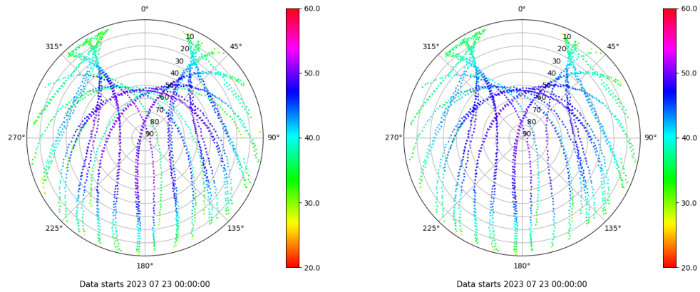
Skyplot for station SEV1. Signal to Noise S1C Data file SEV100ESP_R_2023204.xtr Skyplot for station SEV1. Signal to Noise S2C Data file SEV100ESP_R_2023204.xtr
