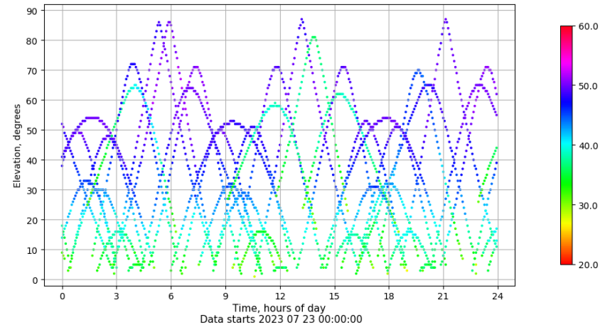
Time-elevation plot for station SEV1. Signal to Noise S1C Data file SEV100ESP_R_2023204.xtr
