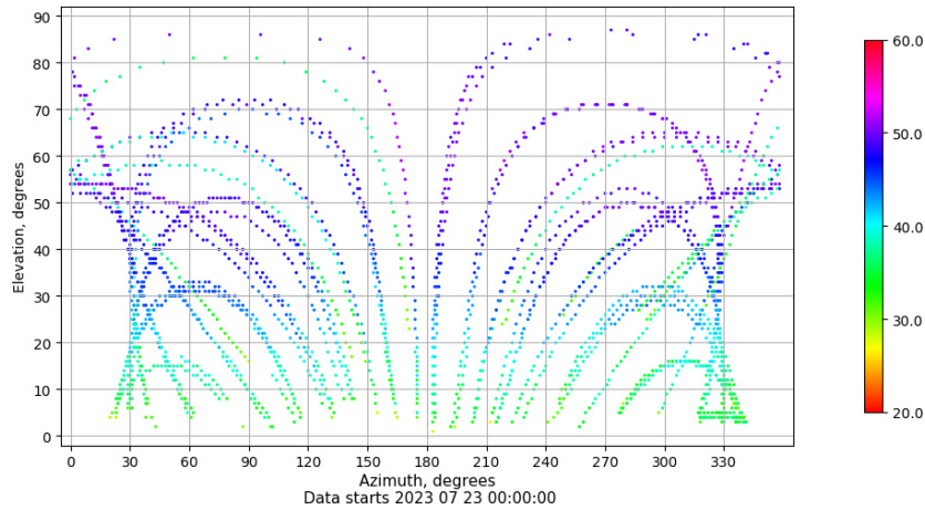
Azimuth-elevation plot for station SEV1. Signal to Noise S1C Data file SEV100ESP_R_2023204.xtr
