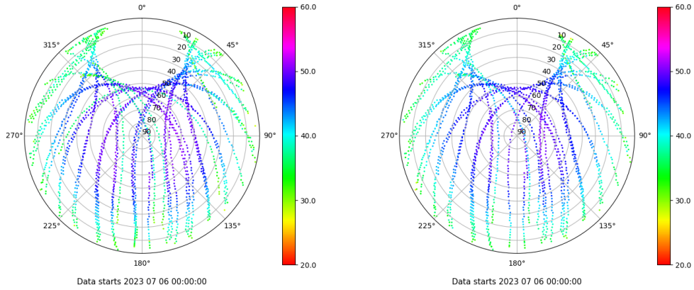
Skyplot for station SEV1. Signal to Noise S1C Data file SEV100ESP_R_2023187.xtr Skyplot for station SEV1. Signal to Noise S2C Data file SEV100ESP_R_2023187.xtr
