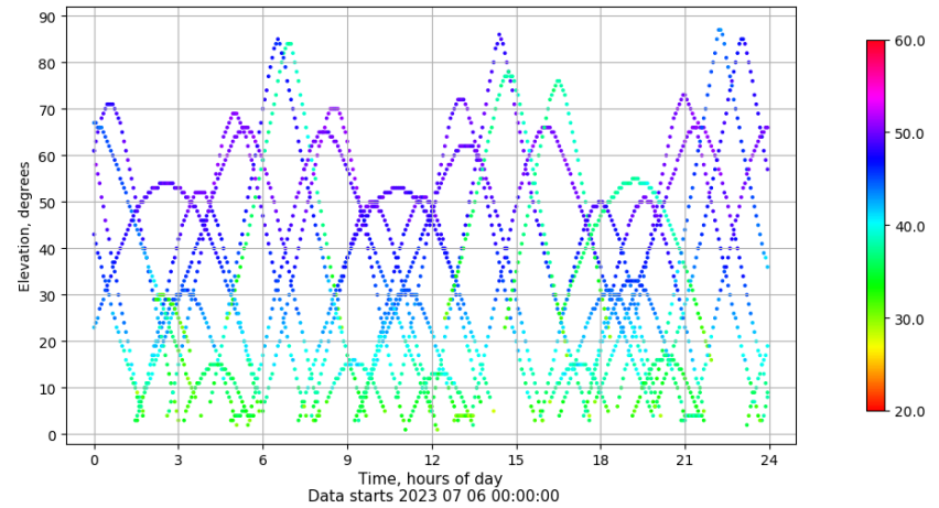
Time-elevation plot for station SEV1. Signal to Noise S1C Data file SEV100ESP_R_2023187.xtr
