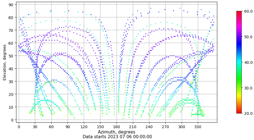
Azimuth-elevation plot for station SEV1. Signal to Noise S1C Data file SEV100ESP_R_2023187.xtr
