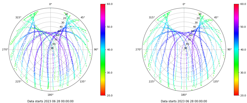
Skyplot for station SEV1. Signal to Noise S1C Data file SEV100ESP_R_2023179.xtr Skyplot for station SEV1. Signal to Noise S2C Data file SEV100ESP_R_2023179.xtr
