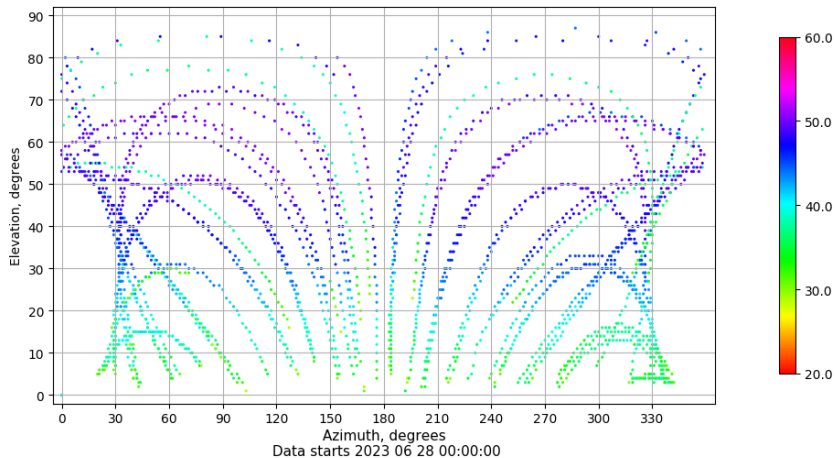
Azimuth-elevation plot for station SEV1. Signal to Noise S1C Data file SEV100ESP_R_2023179.xtr
