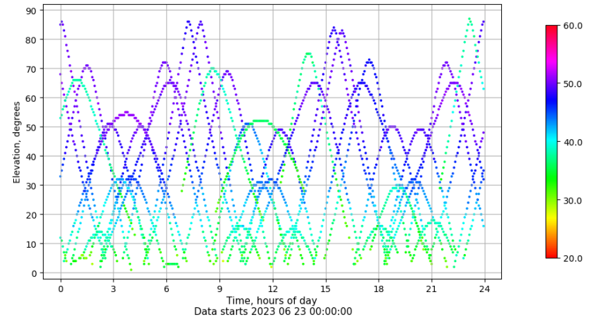
Time-elevation plot for station SEV1. Signal to Noise S1C Data file SEV100ESP_R_2023174.xtr
