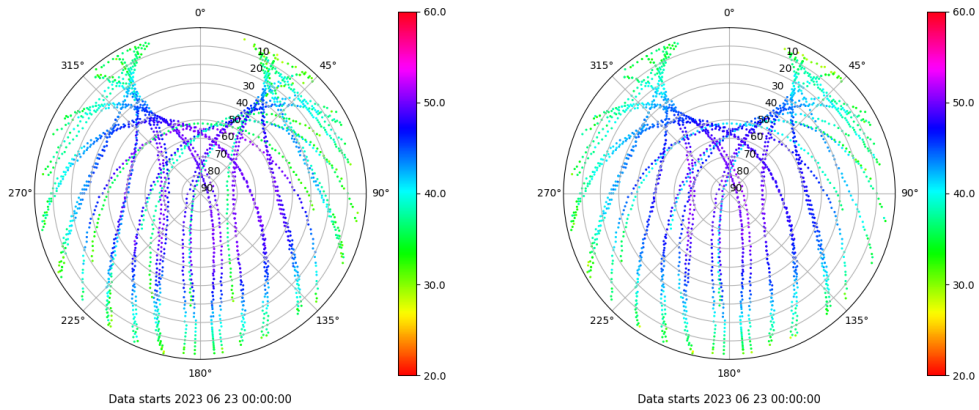
Skyplot for station SEV1. Signal to Noise S1C Data file SEV100ESP_R_2023174.xtr Skyplot for station SEV1. Signal to Noise S2C Data file SEV100ESP_R_2023174.xtr
