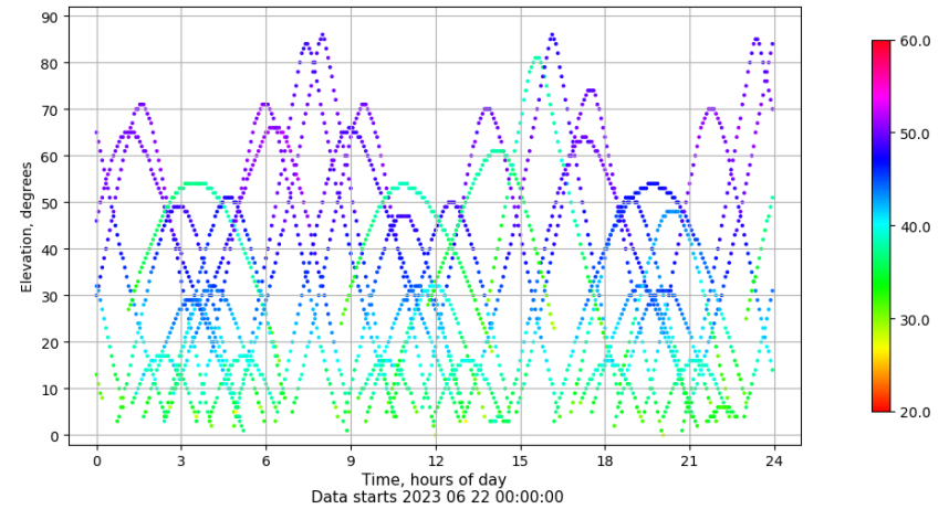
Time-elevation plot for station SEV1. Signal to Noise S1C Data file SEV100ESP_R_2023173.xtr
