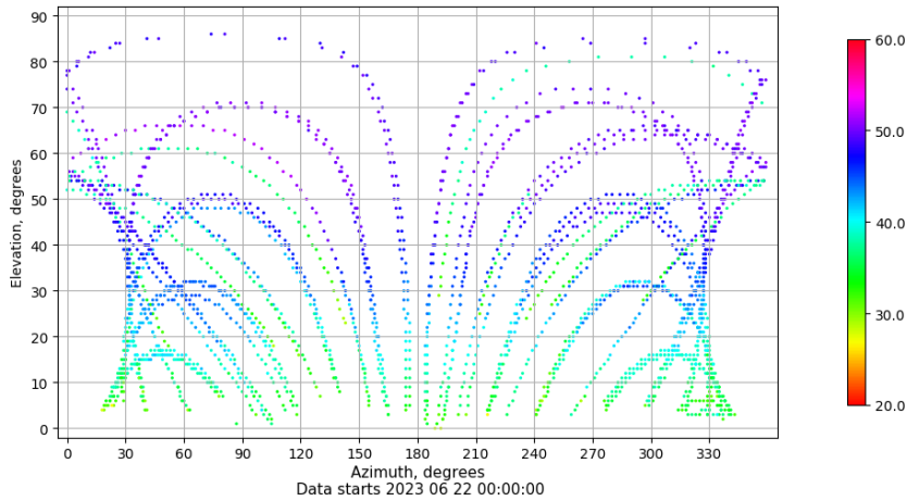
Azimuth-elevation plot for station SEV1. Signal to Noise S1C Data file SEV100ESP_R_2023173.xtr
