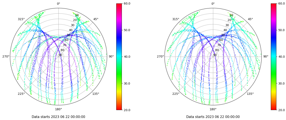
Skyplot for station SEV1. Signal to Noise S1C Data file SEV100ESP_R_2023173.xtr Skyplot for station SEV1. Signal to Noise S2C Data file SEV100ESP_R_2023173.xtr
