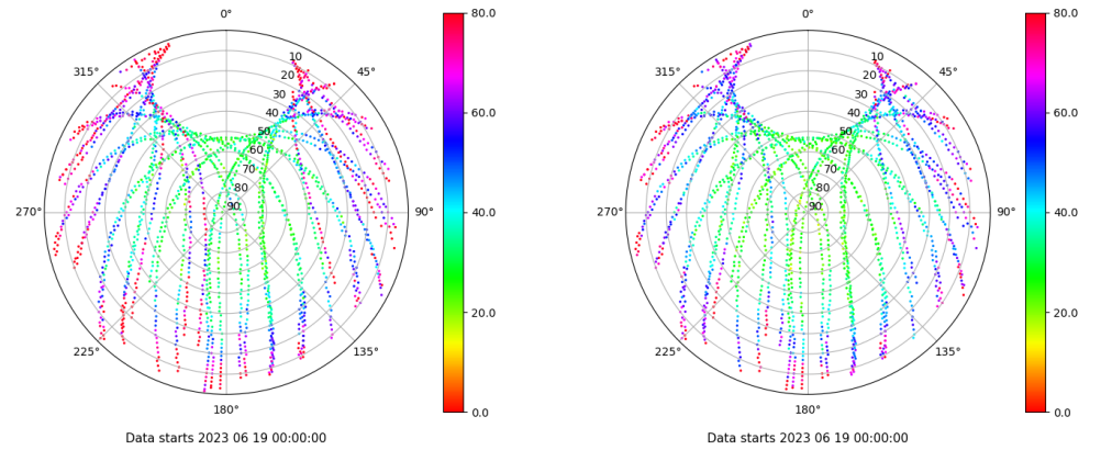
Skyplot for station SEV1. Parameter M1C Data file SEV100ESP_R_2023170.xtr Skyplot for station SEV1. Parameter M2C Data file SEV100ESP_R_2023170.xtr
