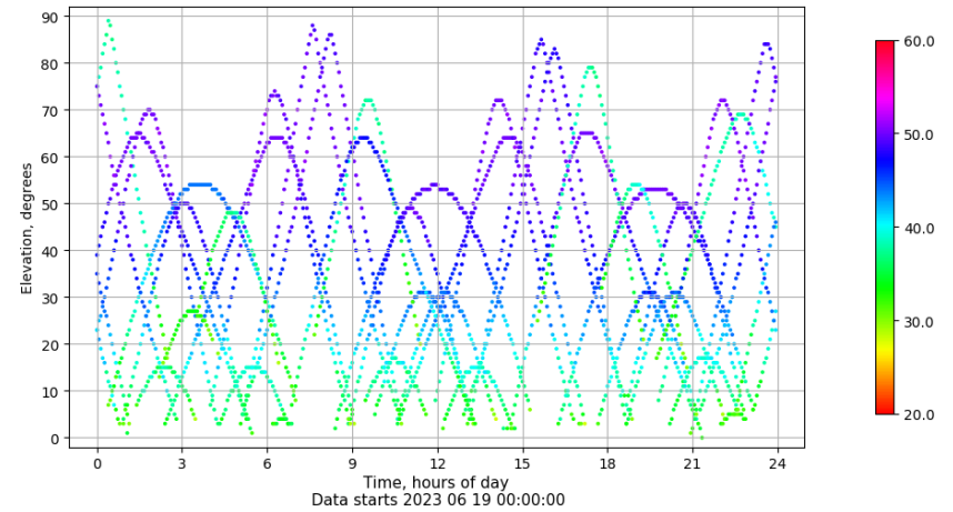
Time-elevation plot for station SEV1. Signal to Noise S1C Data file SEV100ESP_R_2023170.xtr
