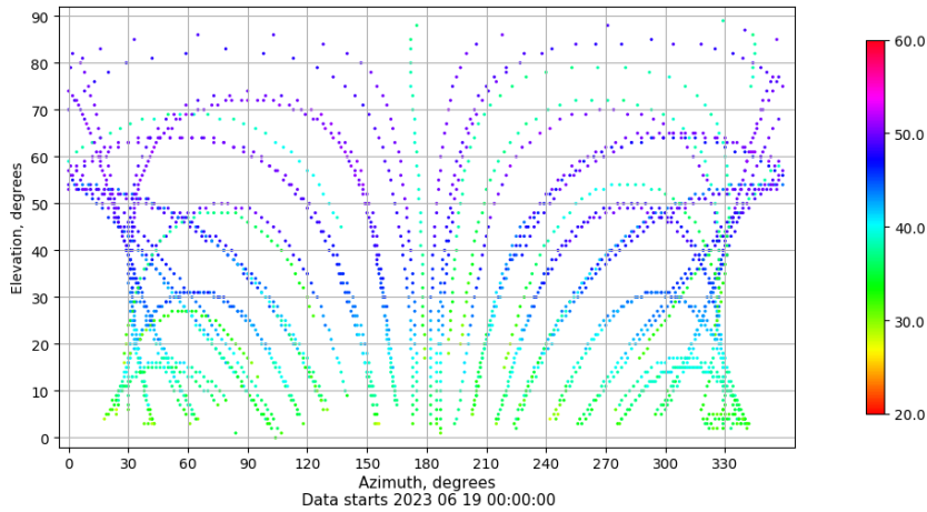
Azimuth-elevation plot for station SEV1. Signal to Noise S1C Data file SEV100ESP_R_2023170.xtr
