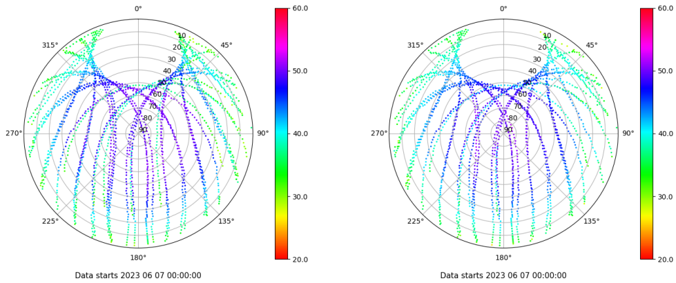
Skyplot for station SEV1. Signal to Noise S1C Data file SEV100ESP_R_2023158.xtr Skyplot for station SEV1. Signal to Noise S2C Data file SEV100ESP_R_2023158.xtr
