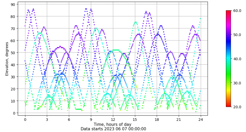
Time-elevation plot for station SEV1. Signal to Noise S1C Data file SEV100ESP_R_2023158.xtr
