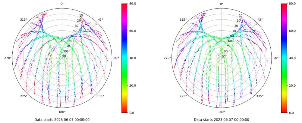
Skyplot for station SEV1. Parameter M1C Data file SEV100ESP_R_2023158.xtr Skyplot for station SEV1. Parameter M2C Data file SEV100ESP_R_2023158.xtr
