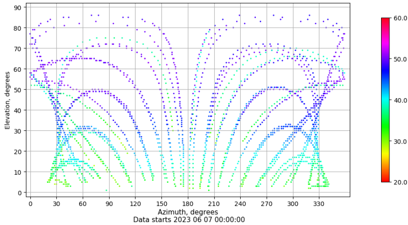
Azimuth-elevation plot for station SEV1. Signal to Noise S1C Data file SEV100ESP_R_2023158.xtr
