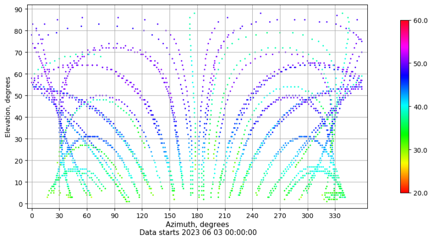
Azimuth-elevation plot for station SEV1. Signal to Noise S1C Data file SEV100ESP_R_2023154.xtr
