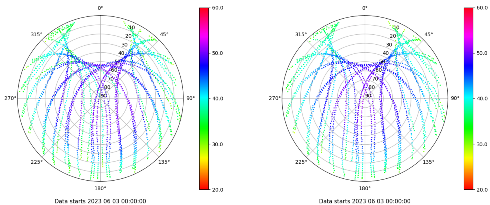
Skyplot for station SEV1. Signal to Noise S1C Data file SEV100ESP_R_2023154.xtr Skyplot for station SEV1. Signal to Noise S2C Data file SEV100ESP_R_2023154.xtr
