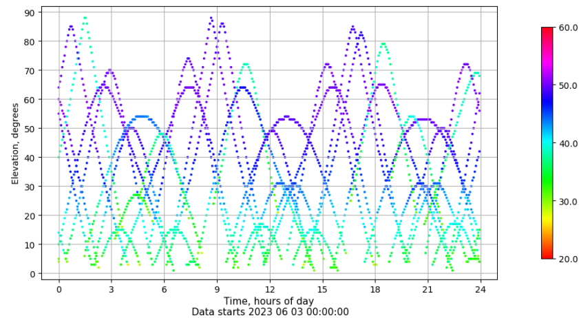
Time-elevation plot for station SEV1. Signal to Noise S1C Data file SEV100ESP_R_2023154.xtr
