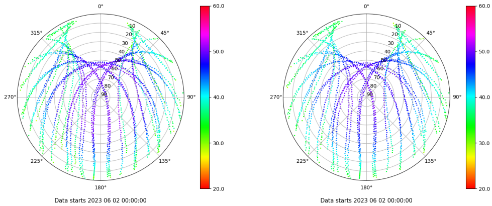
Skyplot for station SEV1. Signal to Noise S1C Data file SEV100ESP_R_2023153.xtr Skyplot for station SEV1. Signal to Noise S2C Data file SEV100ESP_R_2023153.xtr
