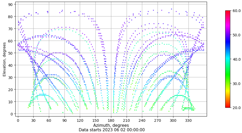
Azimuth-elevation plot for station SEV1. Signal to Noise S1C Data file SEV100ESP_R_2023153.xtr
