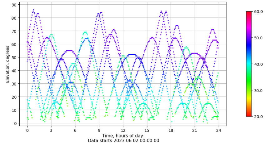
Time-elevation plot for station SEV1. Signal to Noise S1C Data file SEV100ESP_R_2023153.xtr
