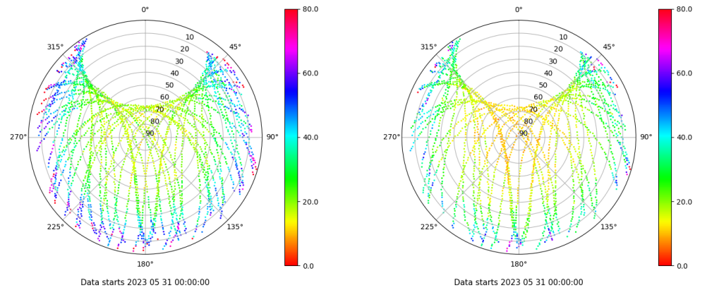
Skyplot for station SEV1. Parameter M1C Data file SEV100ESP_R_2023151.xtr Skyplot for station SEV1. Parameter M2X Data file SEV100ESP_R_2023151.xtr
