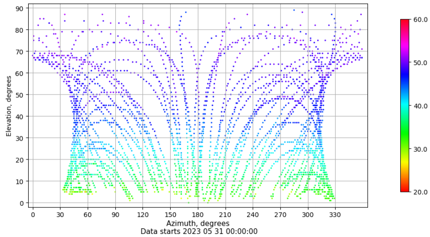
Azimuth-elevation plot for station SEV1. Signal to Noise S1C Data file SEV100ESP_R_2023151.xtr
