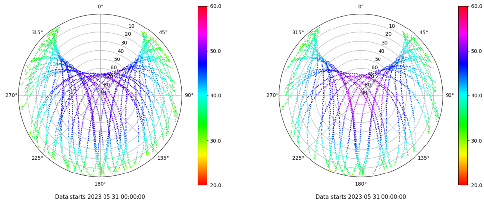
Skyplot for station SEV1. Signal to Noise S1C Data file SEV100ESP_R_2023151.xtr Skyplot for station SEV1. Signal to Noise S2X Data file SEV100ESP_R_2023151.xtr
