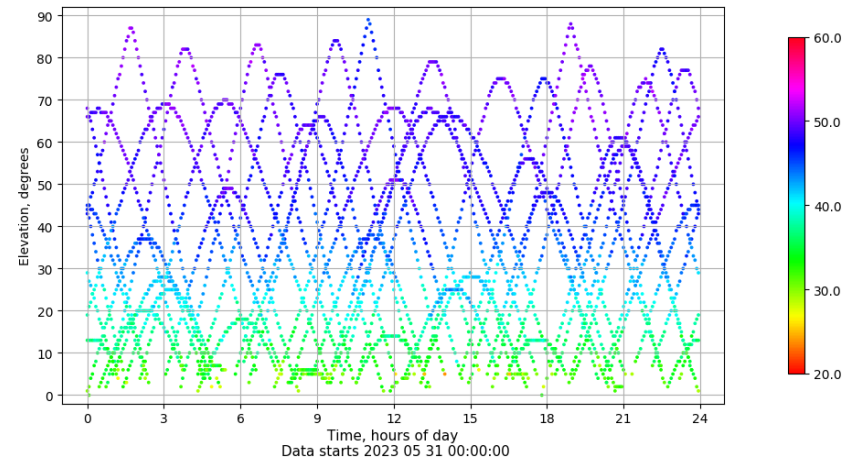
Time-elevation plot for station SEV1. Signal to Noise S1C Data file SEV100ESP_R_2023151.xtr
