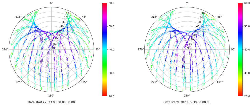
Skyplot for station SEV1. Signal to Noise S1C Data file SEV100ESP_R_2023150.xtr Skyplot for station SEV1. Signal to Noise S2C Data file SEV100ESP_R_2023150.xtr
