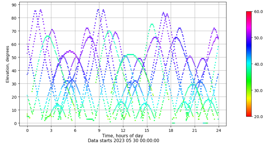
Time-elevation plot for station SEV1. Signal to Noise S1C Data file SEV100ESP_R_2023150.xtr
