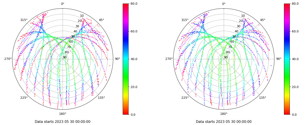
Skyplot for station SEV1. Parameter M1C Data file SEV100ESP_R_2023150.xtr Skyplot for station SEV1. Parameter M2C Data file SEV100ESP_R_2023150.xtr
