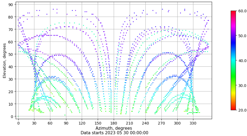
Azimuth-elevation plot for station SEV1. Signal to Noise S1C Data file SEV100ESP_R_2023150.xtr
