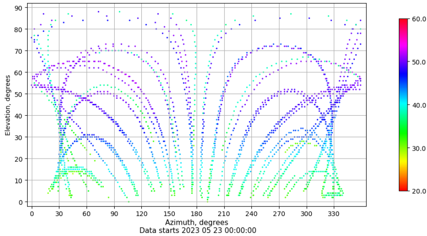
Azimuth-elevation plot for station SEV1. Signal to Noise S1C Data file SEV100ESP_R_2023143.xtr
