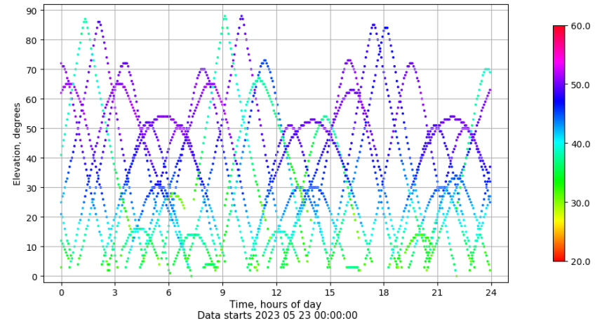
Time-elevation plot for station SEV1. Signal to Noise S1C Data file SEV100ESP_R_2023143.xtr
