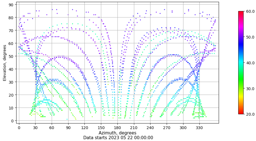
Azimuth-elevation plot for station SEV1. Signal to Noise S1C Data file SEV100ESP_R_2023142.xtr
