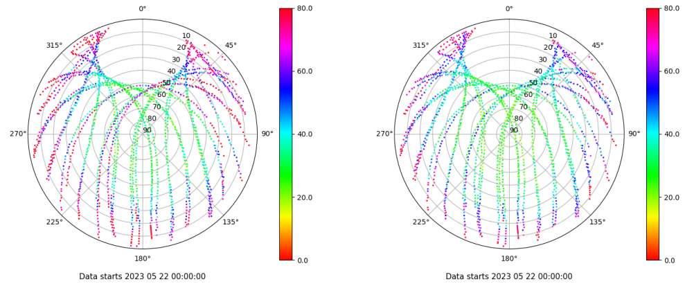
Skyplot for station SEV1. Parameter M1C Data file SEV100ESP_R_2023142.xtr Skyplot for station SEV1. Parameter M2C Data file SEV100ESP_R_2023142.xtr
