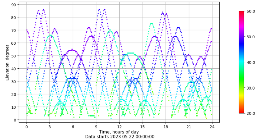
Time-elevation plot for station SEV1. Signal to Noise S1C Data file SEV100ESP_R_2023142.xtr
