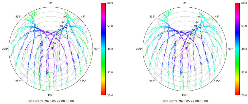
Skyplot for station SEV1. Signal to Noise S1C Data file SEV100ESP_R_2023142.xtr Skyplot for station SEV1. Signal to Noise S2C Data file SEV100ESP_R_2023142.xtr
