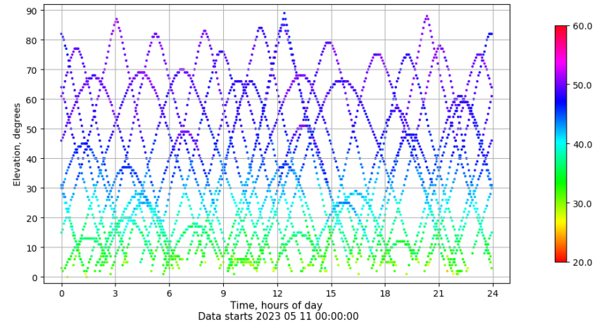
Time-elevation plot for station SEV1. Signal to Noise S1C Data file SEV100ESP_R_2023131.xtr
