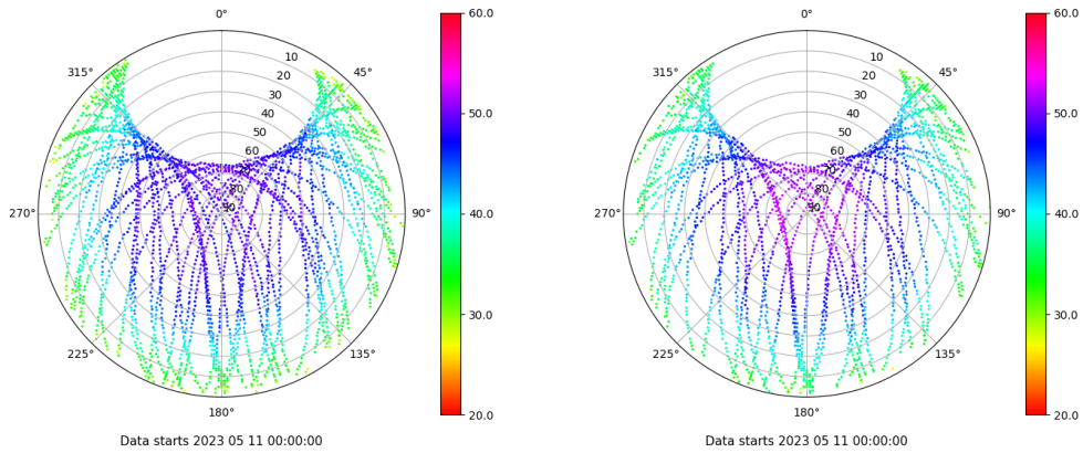
Skyplot for station SEV1. Signal to Noise S1C Data file SEV100ESP_R_2023131.xtr Skyplot for station SEV1. Signal to Noise S2X Data file SEV100ESP_R_2023131.xtr
