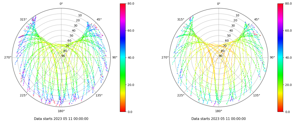
Skyplot for station SEV1. Parameter M1C Data file SEV100ESP_R_2023131.xtr Skyplot for station SEV1. Parameter M2X Data file SEV100ESP_R_2023131.xtr
