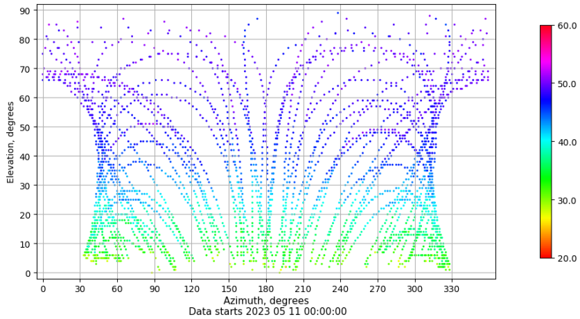
Azimuth-elevation plot for station SEV1. Signal to Noise S1C Data file SEV100ESP_R_2023131.xtr
