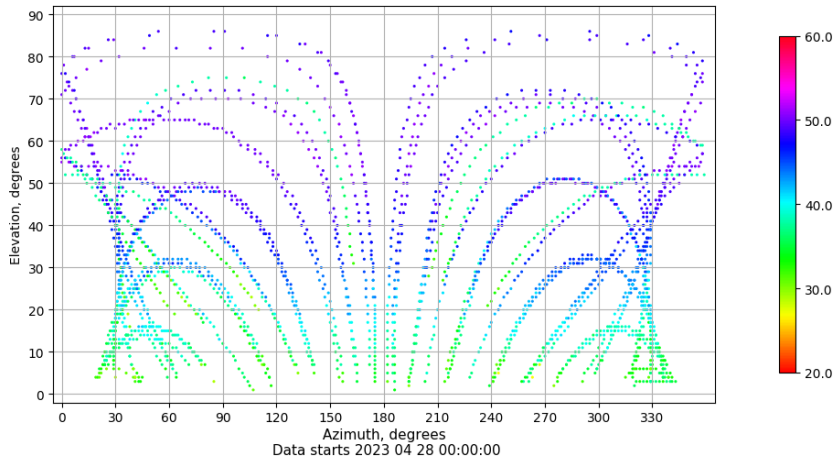
Azimuth-elevation plot for station SEV1. Signal to Noise S1C Data file SEV100ESP_R_2023118.xtr
