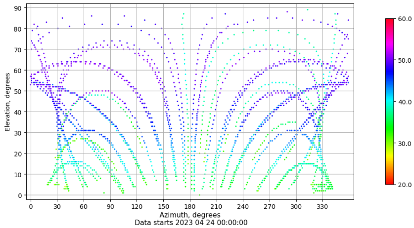
Azimuth-elevation plot for station SEV1. Signal to Noise S1C Data file SEV100ESP_R_2023114.xtr
