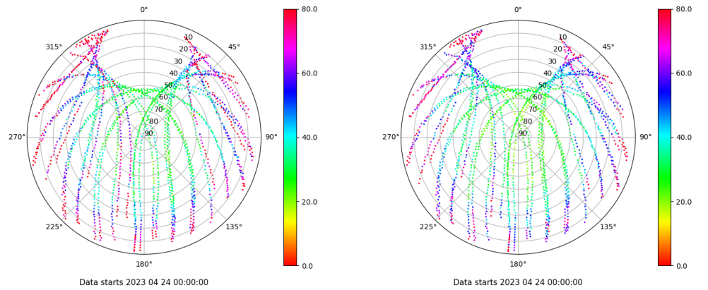
Skyplot for station SEV1. Parameter M1C Data file SEV100ESP_R_2023114.xtr Skyplot for station SEV1. Parameter M2C Data file SEV100ESP_R_2023114.xtr
