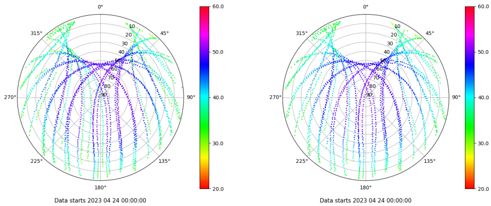
Skyplot for station SEV1. Signal to Noise S1C Data file SEV100ESP_R_2023114.xtr Skyplot for station SEV1. Signal to Noise S2C Data file SEV100ESP_R_2023114.xtr
