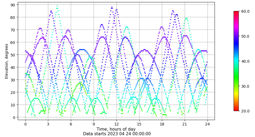
Time-elevation plot for station SEV1. Signal to Noise S1C Data file SEV100ESP_R_2023114.xtr
