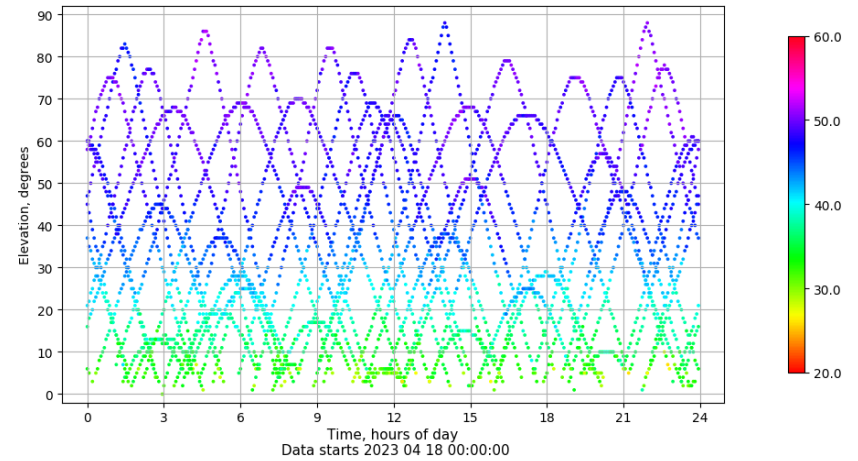
Time-elevation plot for station SEV1. Signal to Noise S1C Data file SEV100ESP_R_2023108.xtr
