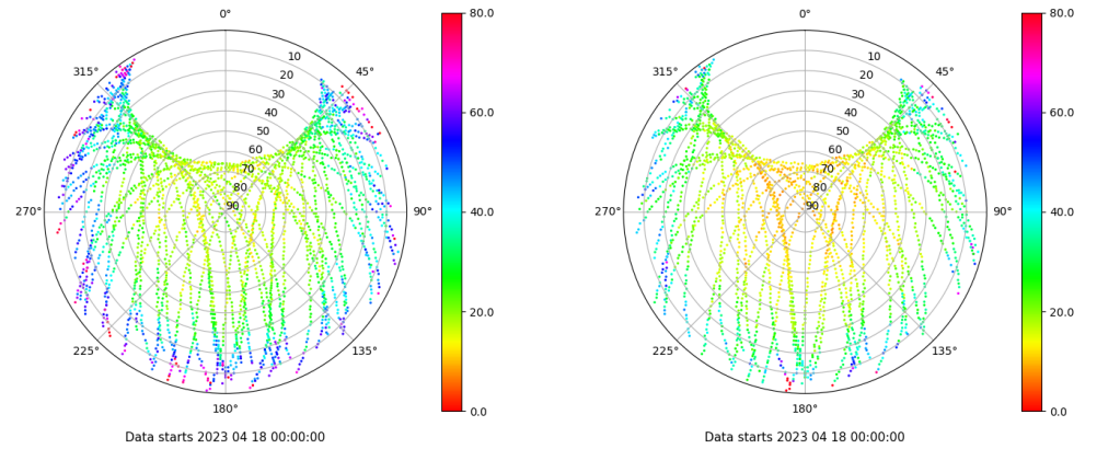
Skyplot for station SEV1. Parameter M1C Data file SEV100ESP_R_2023108.xtr Skyplot for station SEV1. Parameter M2X Data file SEV100ESP_R_2023108.xtr
