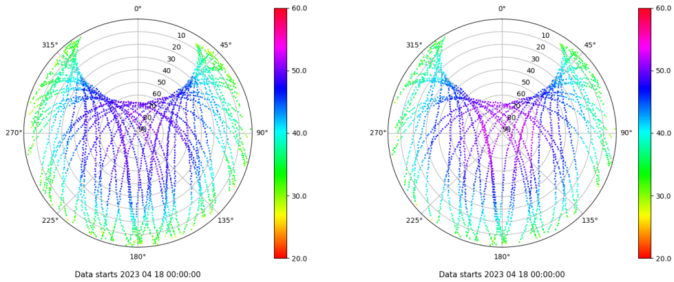
Skyplot for station SEV1. Signal to Noise S1C Data file SEV100ESP_R_2023108.xtr Skyplot for station SEV1. Signal to Noise S2X Data file SEV100ESP_R_2023108.xtr
