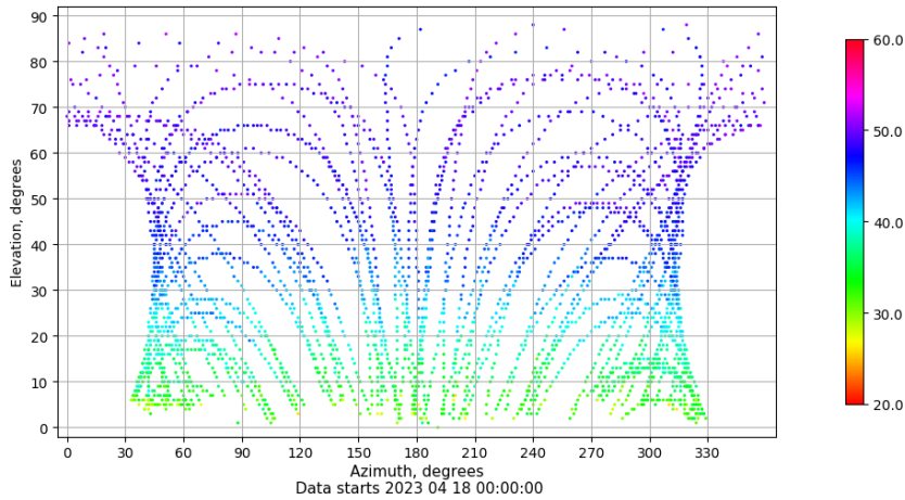
Azimuth-elevation plot for station SEV1. Signal to Noise S1C Data file SEV100ESP_R_2023108.xtr
