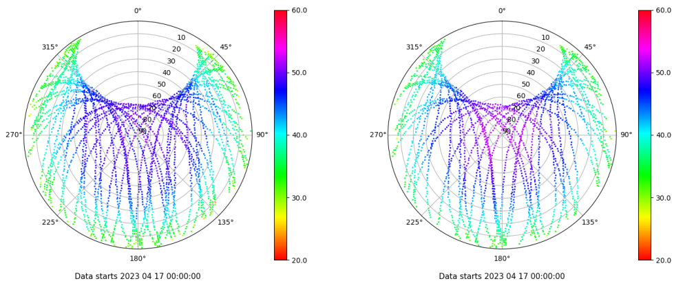
Skyplot for station SEV1. Signal to Noise S1C Data file SEV100ESP_R_2023107.xtr Skyplot for station SEV1. Signal to Noise S2X Data file SEV100ESP_R_2023107.xtr
