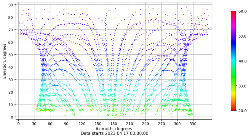
Azimuth-elevation plot for station SEV1. Signal to Noise S1C Data file SEV100ESP_R_2023107.xtr
