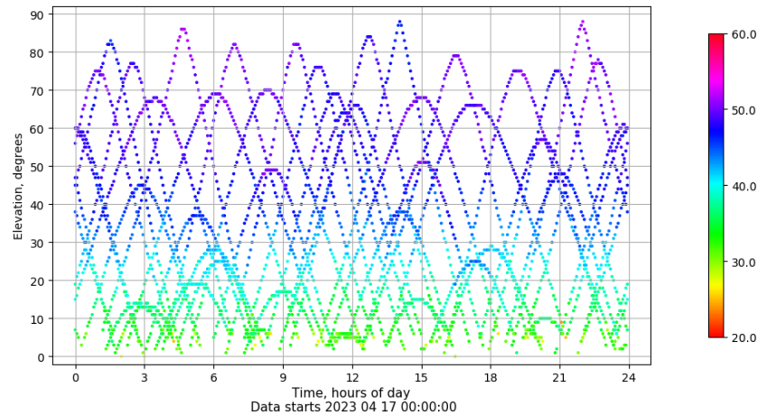
Time-elevation plot for station SEV1. Signal to Noise S1C Data file SEV100ESP_R_2023107.xtr
