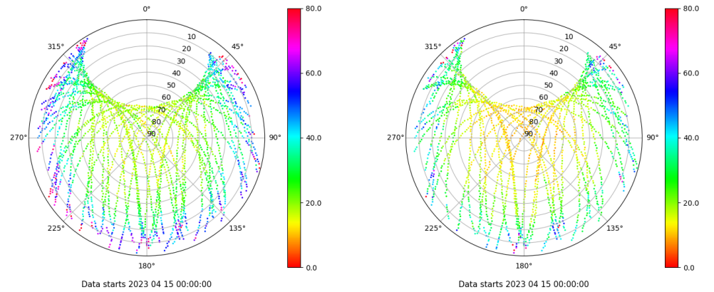
Skyplot for station SEV1. Parameter M1C Data file SEV100ESP_R_2023105.xtr Skyplot for station SEV1. Parameter M2X Data file SEV100ESP_R_2023105.xtr
