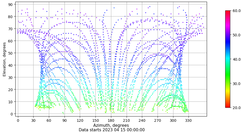
Azimuth-elevation plot for station SEV1. Signal to Noise S1C Data file SEV100ESP_R_2023105.xtr
