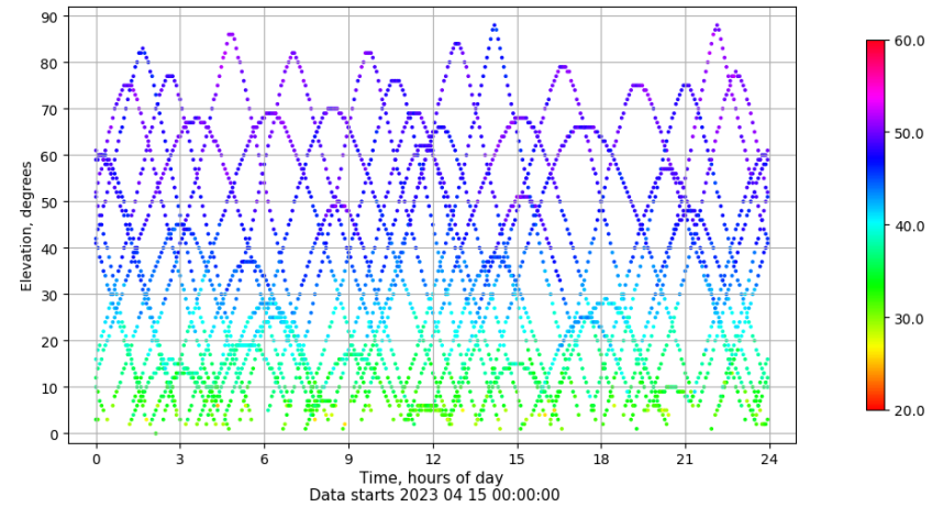
Time-elevation plot for station SEV1. Signal to Noise S1C Data file SEV100ESP_R_2023105.xtr
