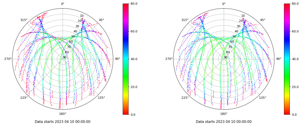
Skyplot for station SEV1. Parameter M1C Data file SEV100ESP_R_2023100.xtr Skyplot for station SEV1. Parameter M2C Data file SEV100ESP_R_2023100.xtr
