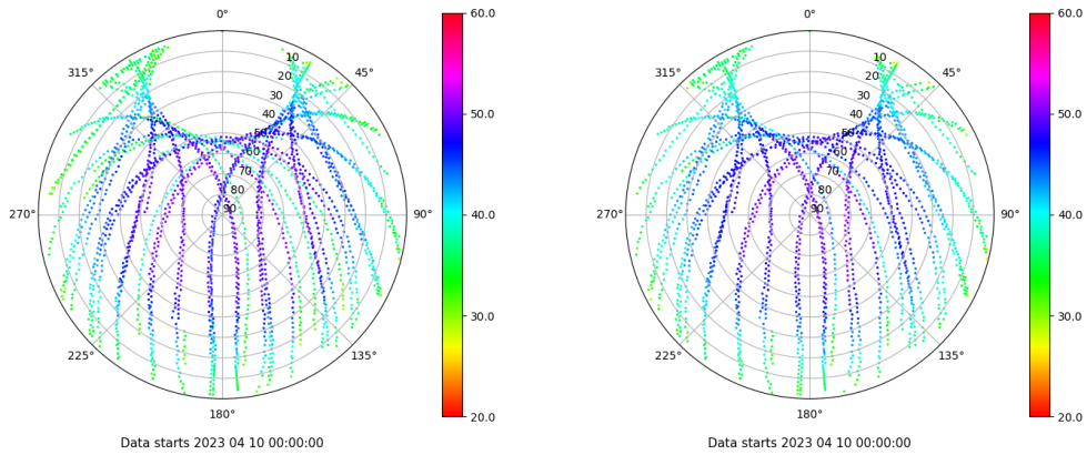
Skyplot for station SEV1. Signal to Noise S1C Data file SEV100ESP_R_2023100.xtr Skyplot for station SEV1. Signal to Noise S2C Data file SEV100ESP_R_2023100.xtr
