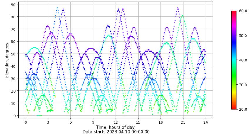
Time-elevation plot for station SEV1. Signal to Noise S1C Data file SEV100ESP_R_2023100.xtr
