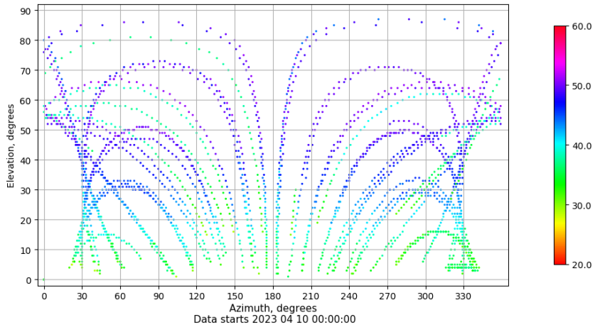
Azimuth-elevation plot for station SEV1. Signal to Noise S1C Data file SEV100ESP_R_2023100.xtr
