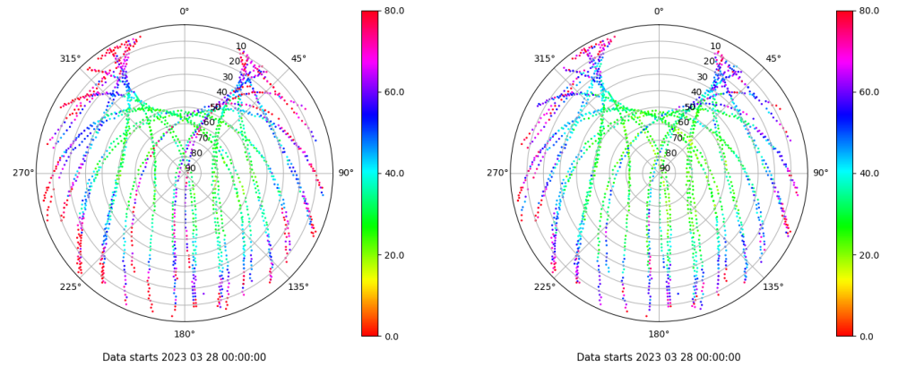
Skyplot for station SEV1. Parameter M1C Data file SEV100ESP_R_2023087.xtr Skyplot for station SEV1. Parameter M2C Data file SEV100ESP_R_2023087.xtr
