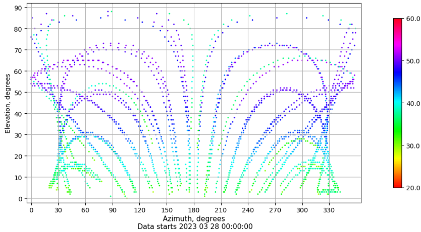
Azimuth-elevation plot for station SEV1. Signal to Noise S1C Data file SEV100ESP_R_2023087.xtr
