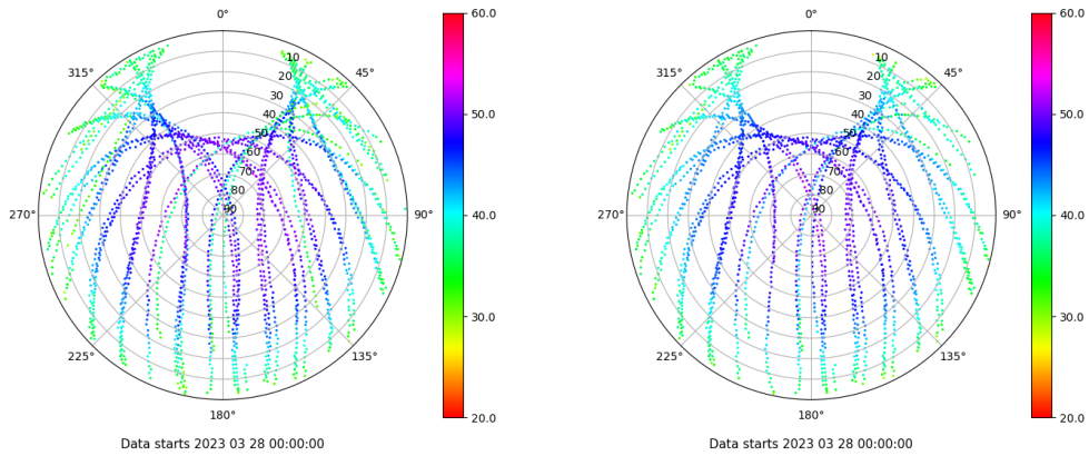
Skyplot for station SEV1. Signal to Noise S1C Data file SEV100ESP_R_2023087.xtr Skyplot for station SEV1. Signal to Noise S2C Data file SEV100ESP_R_2023087.xtr
