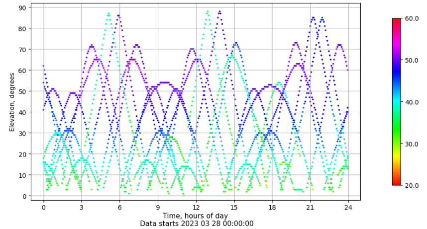
Time-elevation plot for station SEV1. Signal to Noise S1C Data file SEV100ESP_R_2023087.xtr
