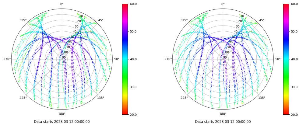
Skyplot for station SEV1. Signal to Noise S1C Data file SEV100ESP_R_2023071.xtr Skyplot for station SEV1. Signal to Noise S2C Data file SEV100ESP_R_2023071.xtr
