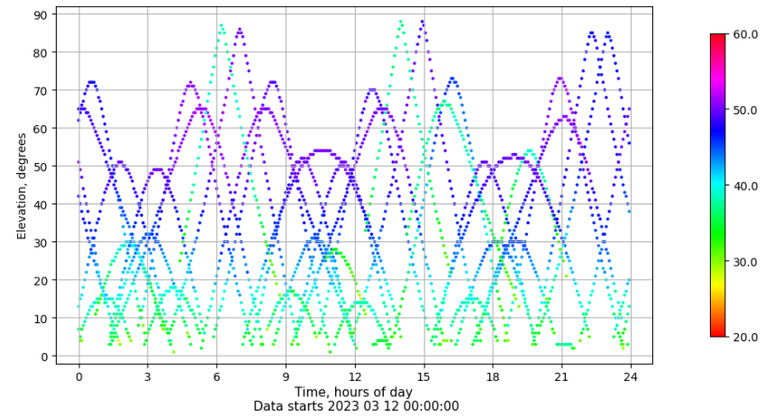
Time-elevation plot for station SEV1. Signal to Noise S1C Data file SEV100ESP_R_2023071.xtr
