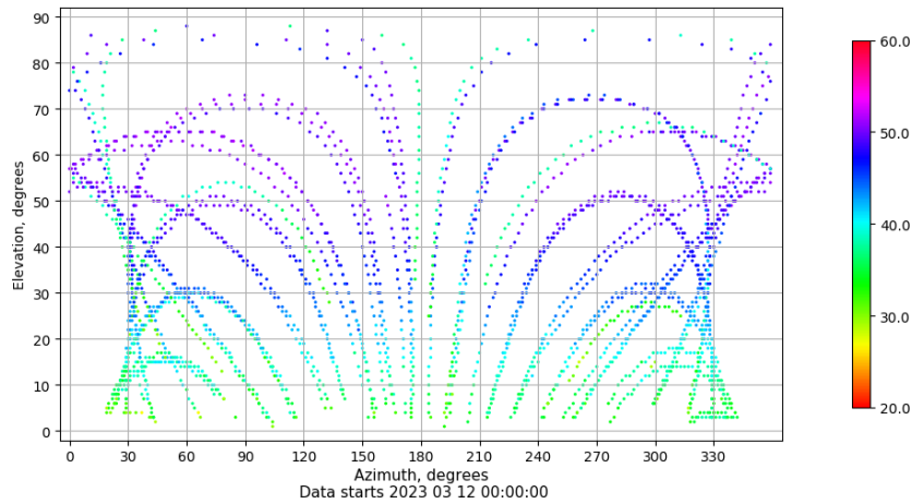
Azimuth-elevation plot for station SEV1. Signal to Noise S1C Data file SEV100ESP_R_2023071.xtr
