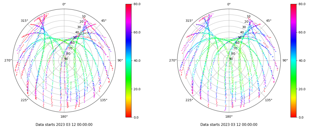
Skyplot for station SEV1. Parameter M1C Data file SEV100ESP_R_2023071.xtr Skyplot for station SEV1. Parameter M2C Data file SEV100ESP_R_2023071.xtr
