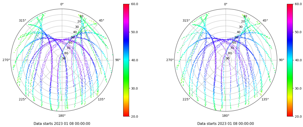
Skyplot for station SEV1. Signal to Noise S1C Data file SEV100ESP_R_2023008.xtr Skyplot for station SEV1. Signal to Noise S2C Data file SEV100ESP_R_2023008.xtr
