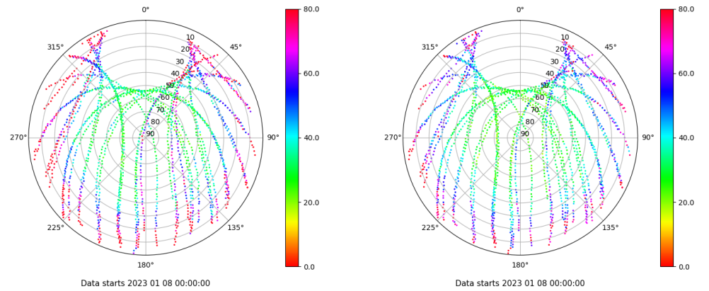
Skyplot for station SEV1. Parameter M1C Data file SEV100ESP_R_2023008.xtr Skyplot for station SEV1. Parameter M2C Data file SEV100ESP_R_2023008.xtr
