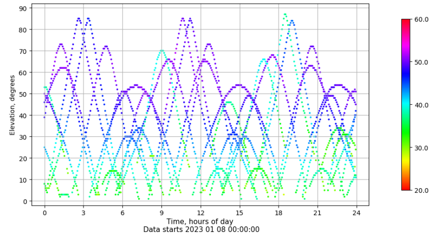
Time-elevation plot for station SEV1. Signal to Noise S1C Data file SEV100ESP_R_2023008.xtr
