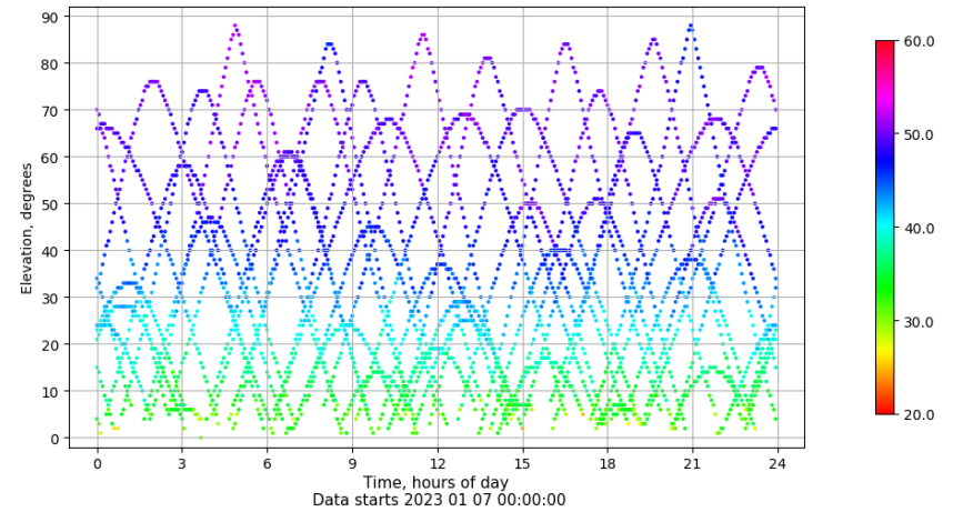
Time-elevation plot for station SEV1. Signal to Noise S1C Data file SEV100ESP_R_2023007.xtr
