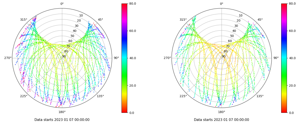
Skyplot for station SEV1. Parameter M1C Data file SEV100ESP_R_2023007.xtr Skyplot for station SEV1. Parameter M2X Data file SEV100ESP_R_2023007.xtr
