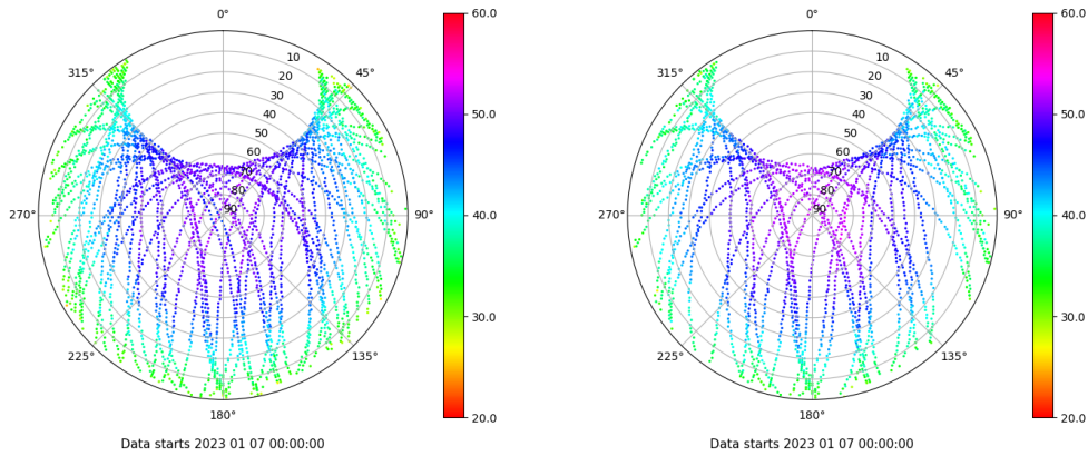
Skyplot for station SEV1. Signal to Noise S1C Data file SEV100ESP_R_2023007.xtr Skyplot for station SEV1. Signal to Noise S2X Data file SEV100ESP_R_2023007.xtr
