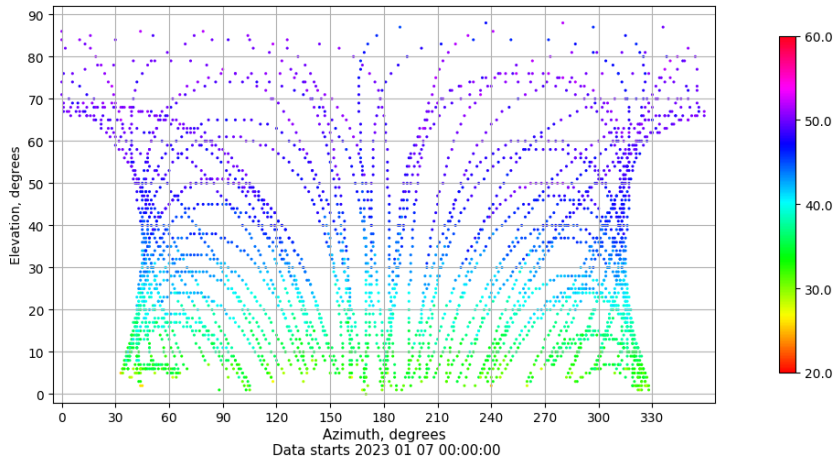
Azimuth-elevation plot for station SEV1. Signal to Noise S1C Data file SEV100ESP_R_2023007.xtr
