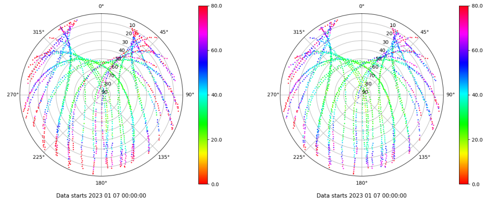
Skyplot for station SEV1. Parameter M1C Data file SEV100ESP_R_2023007.xtr Skyplot for station SEV1. Parameter M2C Data file SEV100ESP_R_2023007.xtr
