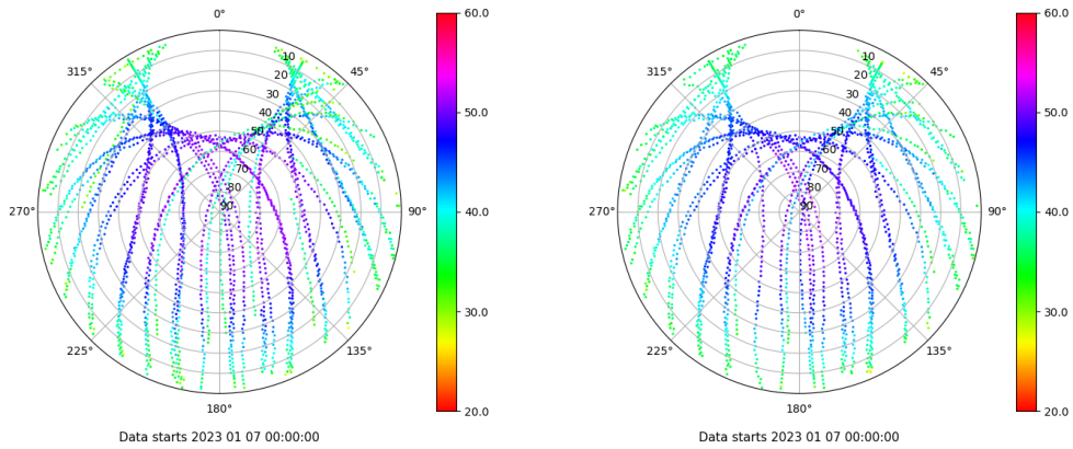
Skyplot for station SEV1. Signal to Noise S1C Data file SEV100ESP_R_2023007.xtr Skyplot for station SEV1. Signal to Noise S2C Data file SEV100ESP_R_2023007.xtr
