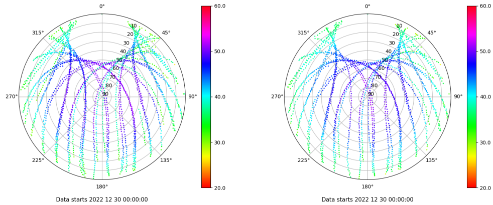
Skyplot for station SEV1. Signal to Noise S1C Data file SEV100ESP_R_2022364.xtr Skyplot for station SEV1. Signal to Noise S2C Data file SEV100ESP_R_2022364.xtr
