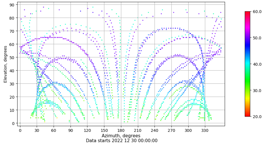
Azimuth-elevation plot for station SEV1. Signal to Noise S1C Data file SEV100ESP_R_2022364.xtr
