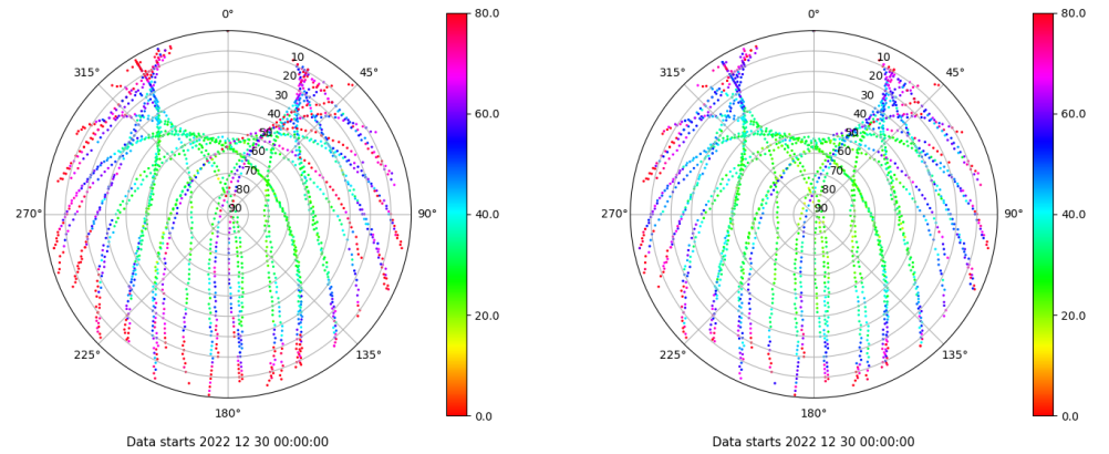
Skyplot for station SEV1. Parameter M1C Data file SEV100ESP_R_2022364.xtr Skyplot for station SEV1. Parameter M2C Data file SEV100ESP_R_2022364.xtr
