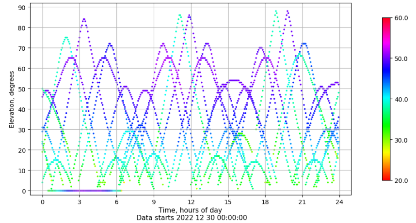
Time-elevation plot for station SEV1. Signal to Noise S1C Data file SEV100ESP_R_2022364.xtr
