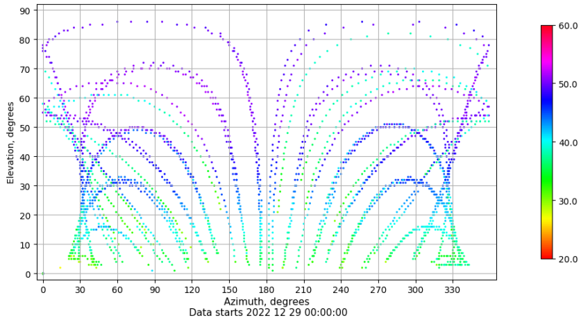
Azimuth-elevation plot for station SEV1. Signal to Noise S1C Data file SEV100ESP_R_2022363.xtr
