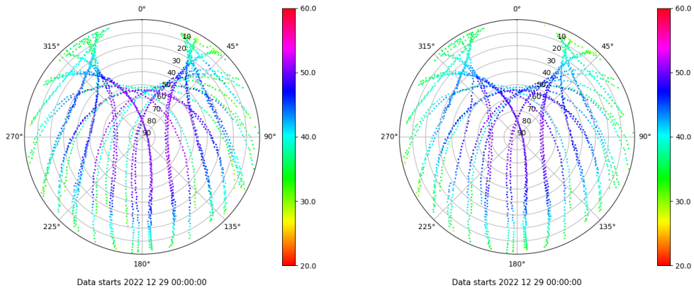
Skyplot for station SEV1. Signal to Noise S1C Data file SEV100ESP_R_2022363.xtr Skyplot for station SEV1. Signal to Noise S2C Data file SEV100ESP_R_2022363.xtr
