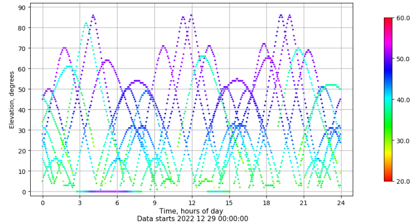
Time-elevation plot for station SEV1. Signal to Noise S1C Data file SEV100ESP_R_2022363.xtr
