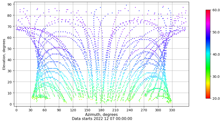
Azimuth-elevation plot for station SEV1. Signal to Noise S1C Data file SEV100ESP_R_2022341.xtr
