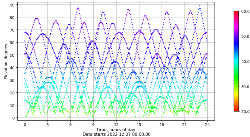
Time-elevation plot for station SEV1. Signal to Noise S1C Data file SEV100ESP_R_2022341.xtr
