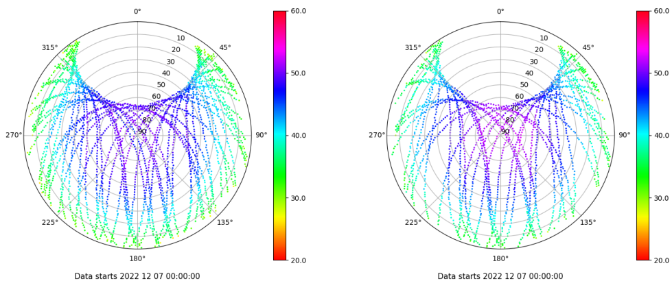
Skyplot for station SEV1. Signal to Noise S1C Data file SEV100ESP_R_2022341.xtr Skyplot for station SEV1. Signal to Noise S2X Data file SEV100ESP_R_2022341.xtr
