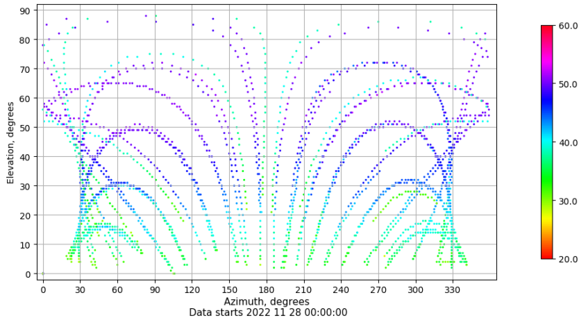
Azimuth-elevation plot for station SEV1. Signal to Noise S1C Data file SEV100ESP_R_2022332.xtr
