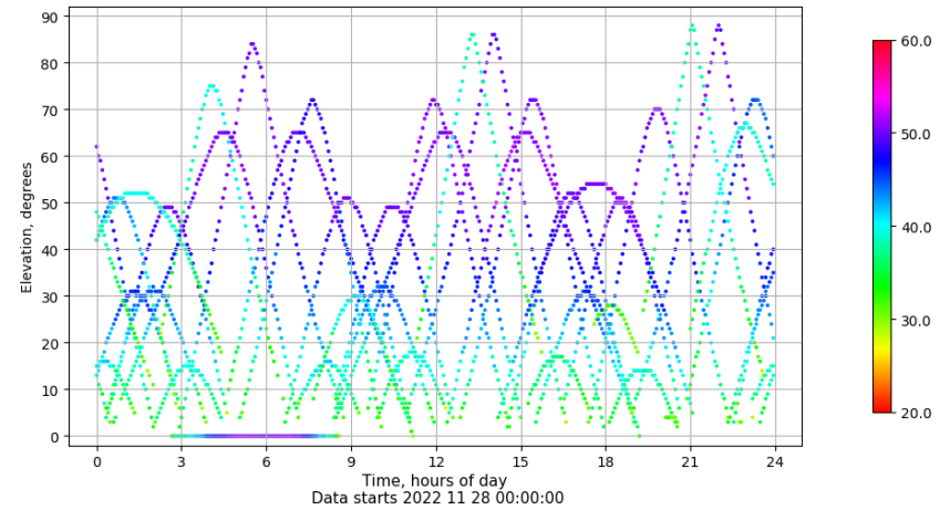
Time-elevation plot for station SEV1. Signal to Noise S1C Data file SEV100ESP_R_2022332.xtr
