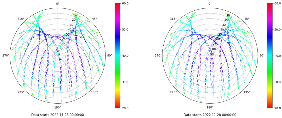
Skyplot for station SEV1. Signal to Noise S1C Data file SEV100ESP_R_2022332.xtr Skyplot for station SEV1. Signal to Noise S2C Data file SEV100ESP_R_2022332.xtr
