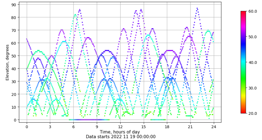
Time-elevation plot for station SEV1. Signal to Noise S1C Data file SEV100ESP_R_2022323.xtr
