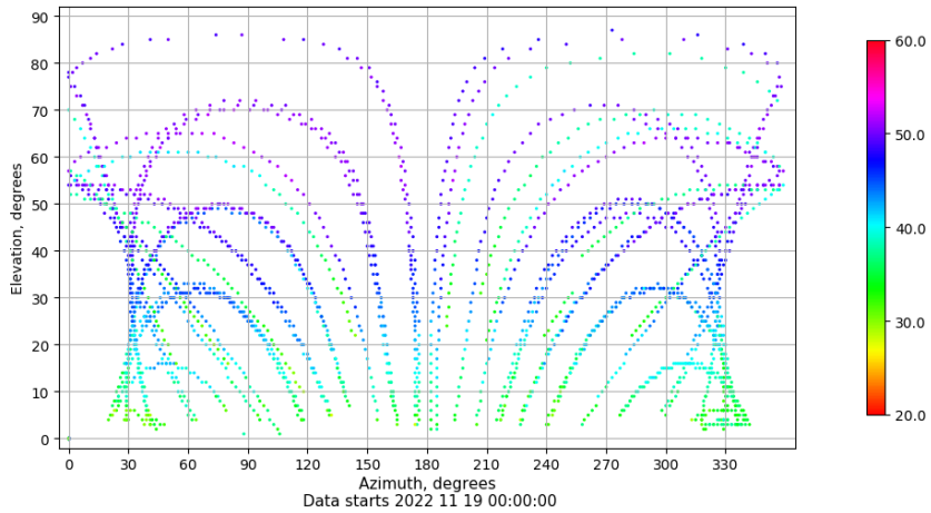
Azimuth-elevation plot for station SEV1. Signal to Noise S1C Data file SEV100ESP_R_2022323.xtr
