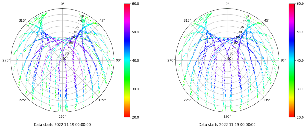
Skyplot for station SEV1. Signal to Noise S1C Data file SEV100ESP_R_2022323.xtr Skyplot for station SEV1. Signal to Noise S2C Data file SEV100ESP_R_2022323.xtr
