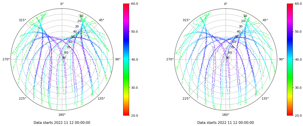
Skyplot for station SEV1. Signal to Noise S1C Data file SEV100ESP_R_2022316.xtr Skyplot for station SEV1. Signal to Noise S2C Data file SEV100ESP_R_2022316.xtr
