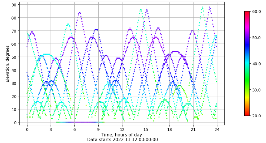
Time-elevation plot for station SEV1. Signal to Noise S1C Data file SEV100ESP_R_2022316.xtr
