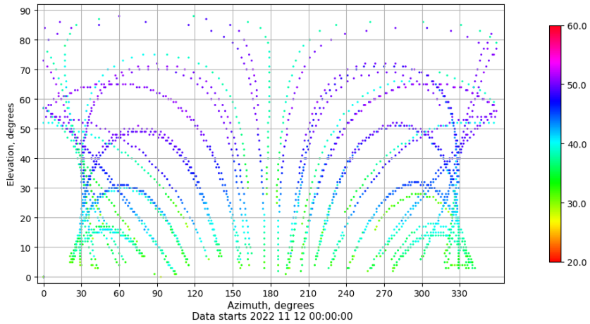
Azimuth-elevation plot for station SEV1. Signal to Noise S1C Data file SEV100ESP_R_2022316.xtr
