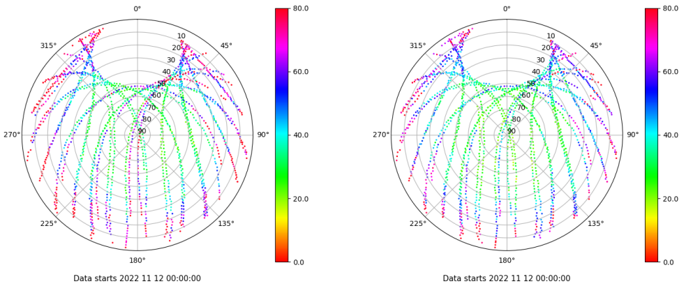
Skyplot for station SEV1. Parameter M1C Data file SEV100ESP_R_2022316.xtr Skyplot for station SEV1. Parameter M2C Data file SEV100ESP_R_2022316.xtr
