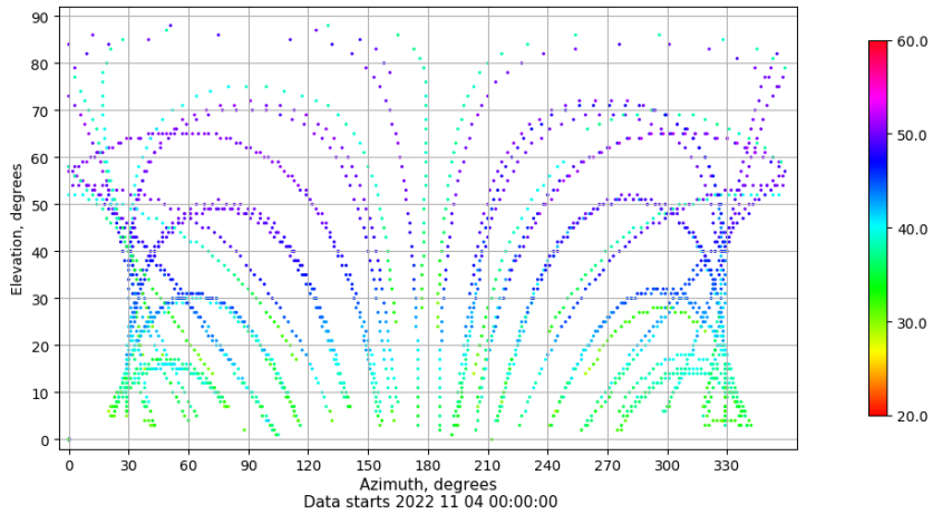
Azimuth-elevation plot for station SEV1. Signal to Noise S1C Data file SEV100ESP_R_2022308.xtr
