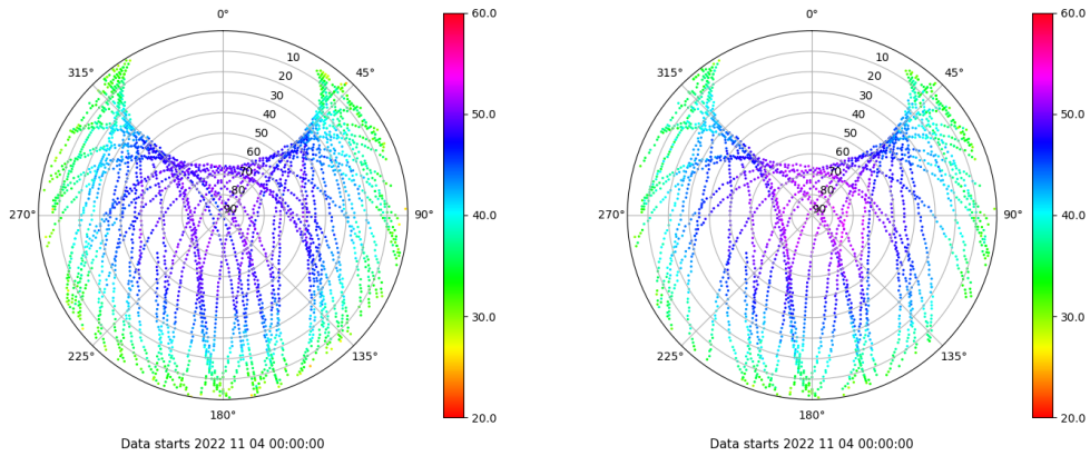
Skyplot for station SEV1. Signal to Noise S1C Data file SEV100ESP_R_2022308.xtr Skyplot for station SEV1. Signal to Noise S2X Data file SEV100ESP_R_2022308.xtr
