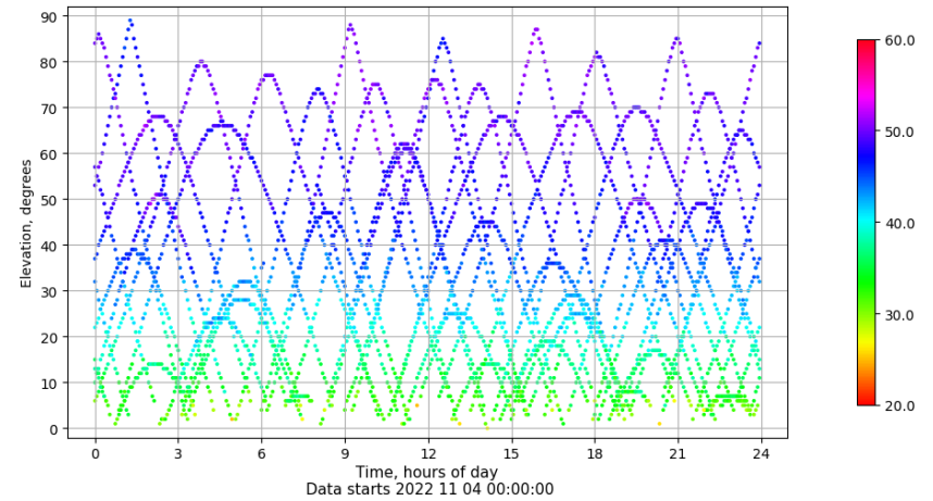
Time-elevation plot for station SEV1. Signal to Noise S1C Data file SEV100ESP_R_2022308.xtr
