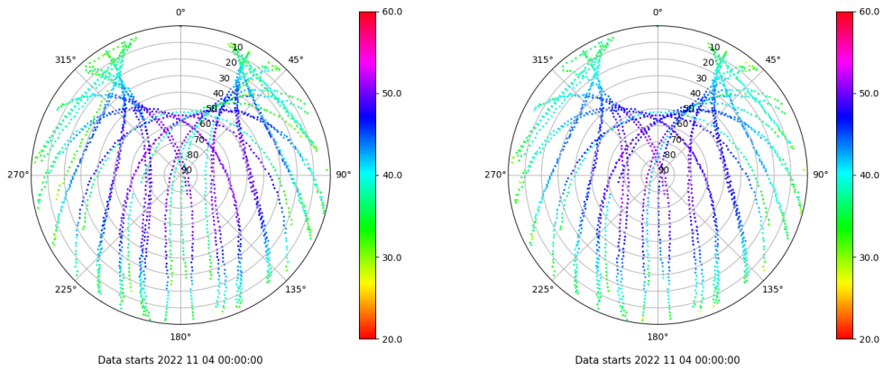
Skyplot for station SEV1. Signal to Noise S1C Data file SEV100ESP_R_2022308.xtr Skyplot for station SEV1. Signal to Noise S2C Data file SEV100ESP_R_2022308.xtr
