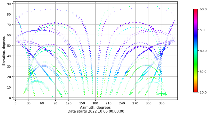
Azimuth-elevation plot for station SEV1. Signal to Noise S1C Data file SEV100ESP_R_2022278.xtr
