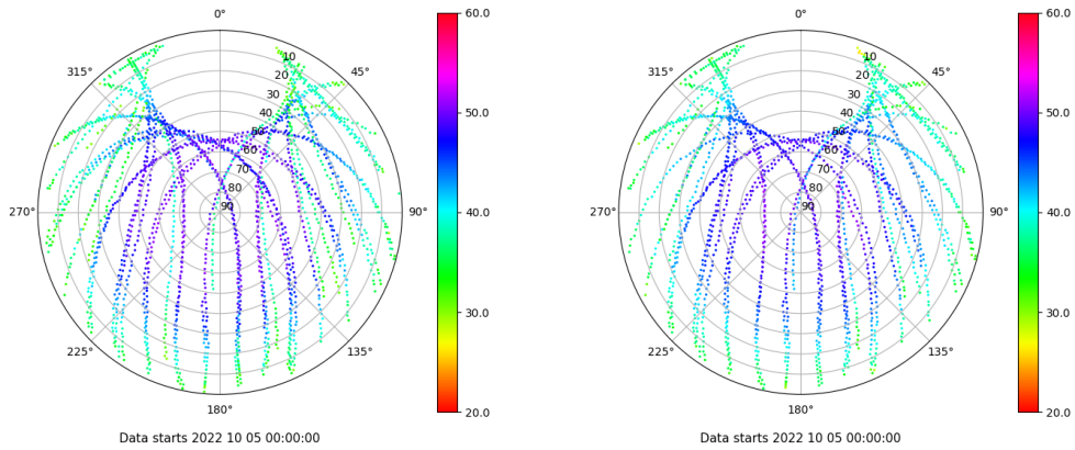
Skyplot for station SEV1. Signal to Noise S1C Data file SEV100ESP_R_2022278.xtr Skyplot for station SEV1. Signal to Noise S2C Data file SEV100ESP_R_2022278.xtr
