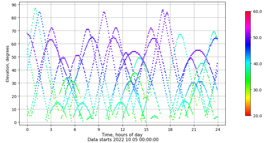
Time-elevation plot for station SEV1. Signal to Noise S1C Data file SEV100ESP_R_2022278.xtr
