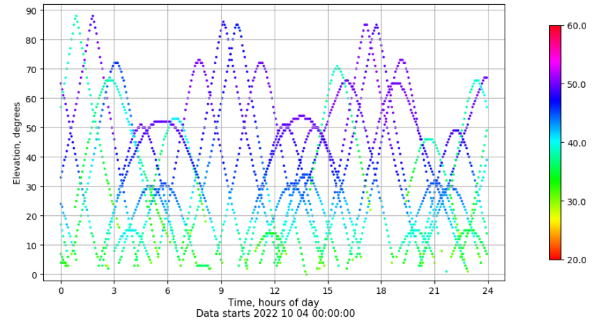
Time-elevation plot for station SEV1. Signal to Noise S1C Data file SEV100ESP_R_2022277.xtr
