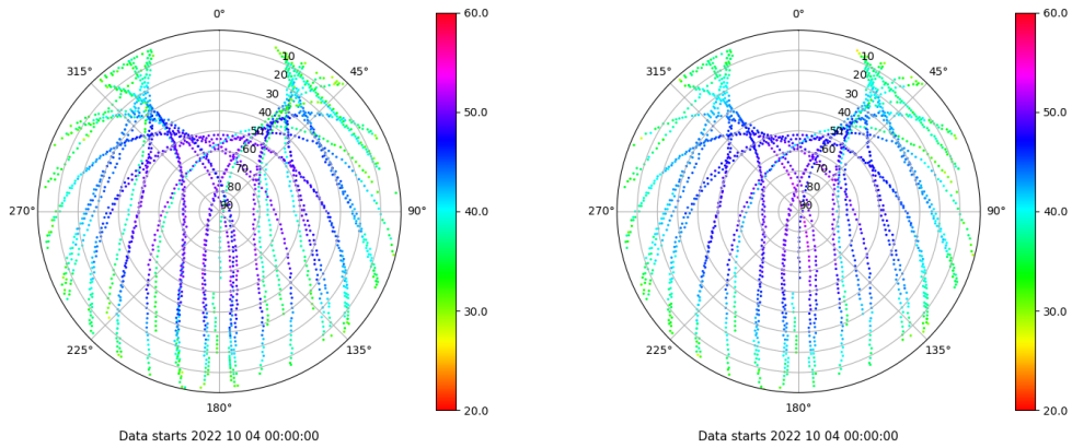
Skyplot for station SEV1. Signal to Noise S1C Data file SEV100ESP_R_2022277.xtr Skyplot for station SEV1. Signal to Noise S2C Data file SEV100ESP_R_2022277.xtr
