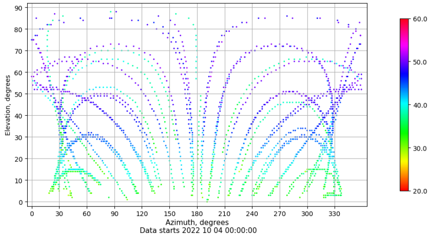
Azimuth-elevation plot for station SEV1. Signal to Noise S1C Data file SEV100ESP_R_2022277.xtr
