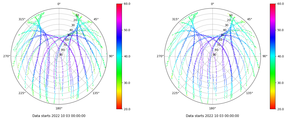
Skyplot for station SEV1. Signal to Noise S1C Data file SEV100ESP_R_2022276.xtr Skyplot for station SEV1. Signal to Noise S2C Data file SEV100ESP_R_2022276.xtr
