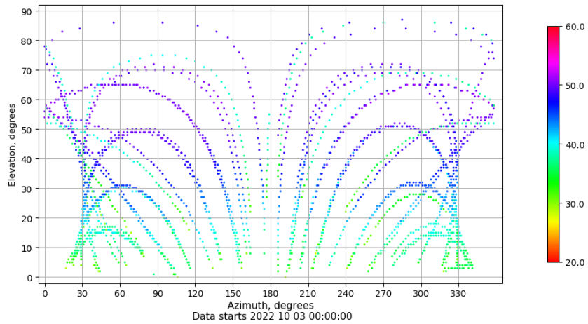
Azimuth-elevation plot for station SEV1. Signal to Noise S1C Data file SEV100ESP_R_2022276.xtr
