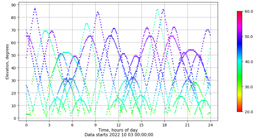
Time-elevation plot for station SEV1. Signal to Noise S1C Data file SEV100ESP_R_2022276.xtr
