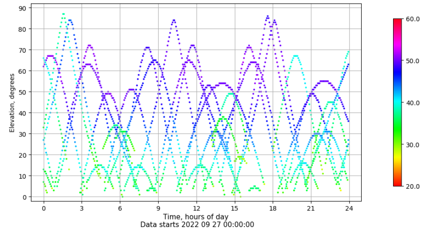
Time-elevation plot for station SEV1. Signal to Noise S1C Data file SEV100ESP_R_2022270.xtr
