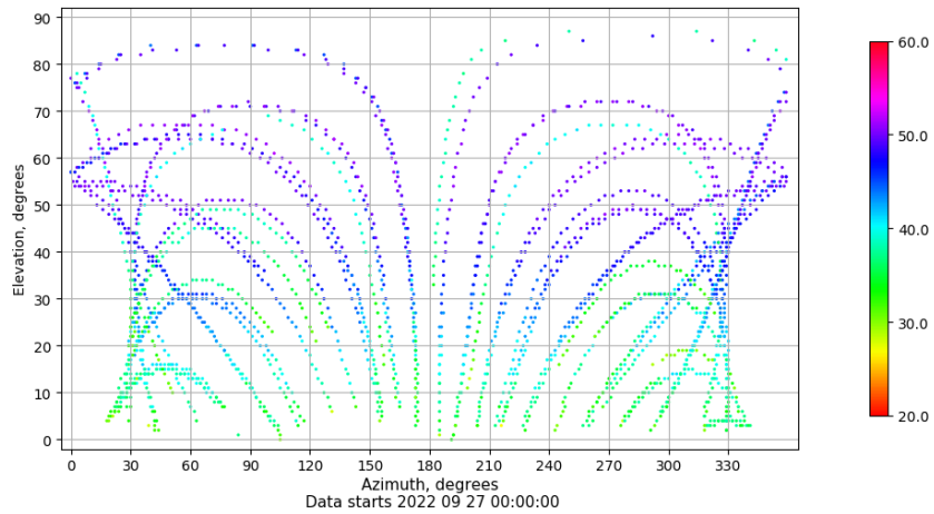
Azimuth-elevation plot for station SEV1. Signal to Noise S1C Data file SEV100ESP_R_2022270.xtr
