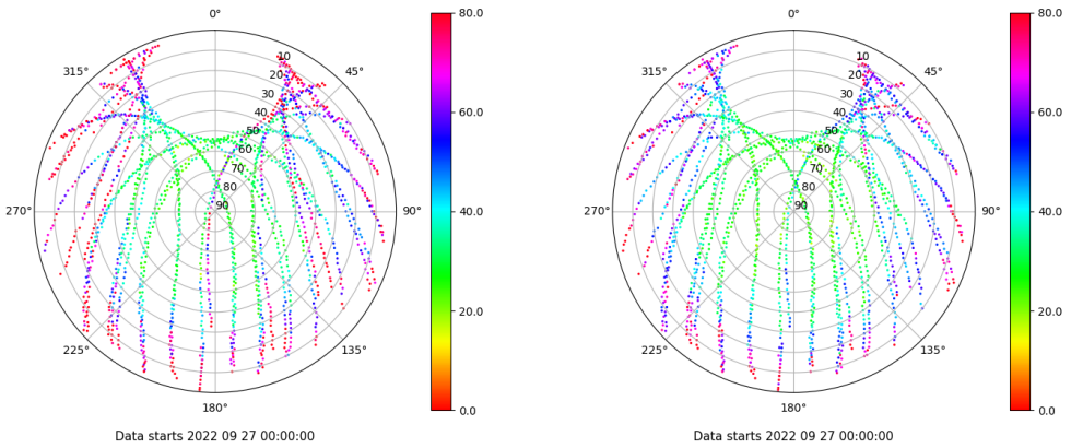
Skyplot for station SEV1. Parameter M1C Data file SEV100ESP_R_2022270.xtr Skyplot for station SEV1. Parameter M2C Data file SEV100ESP_R_2022270.xtr
