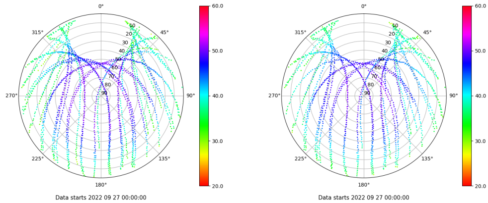
Skyplot for station SEV1. Signal to Noise S1C Data file SEV100ESP_R_2022270.xtr Skyplot for station SEV1. Signal to Noise S2C Data file SEV100ESP_R_2022270.xtr
