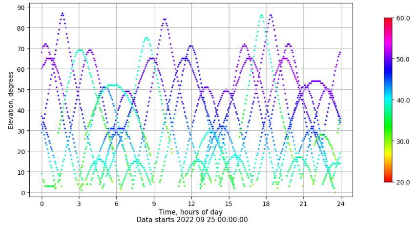
Time-elevation plot for station SEV1. Signal to Noise S1C Data file SEV100ESP_R_2022268.xtr
