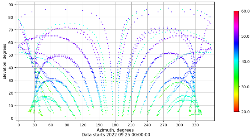
Azimuth-elevation plot for station SEV1. Signal to Noise S1C Data file SEV100ESP_R_2022268.xtr
