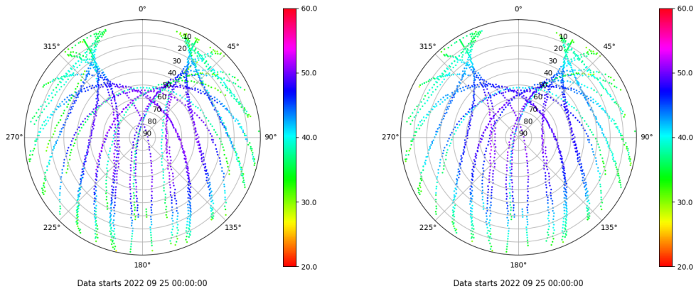
Skyplot for station SEV1. Signal to Noise S1C Data file SEV100ESP_R_2022268.xtr Skyplot for station SEV1. Signal to Noise S2C Data file SEV100ESP_R_2022268.xtr
