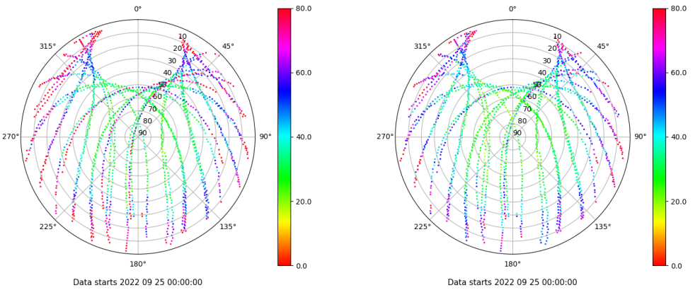
Skyplot for station SEV1. Parameter M1C Data file SEV100ESP_R_2022268.xtr Skyplot for station SEV1. Parameter M2C Data file SEV100ESP_R_2022268.xtr
