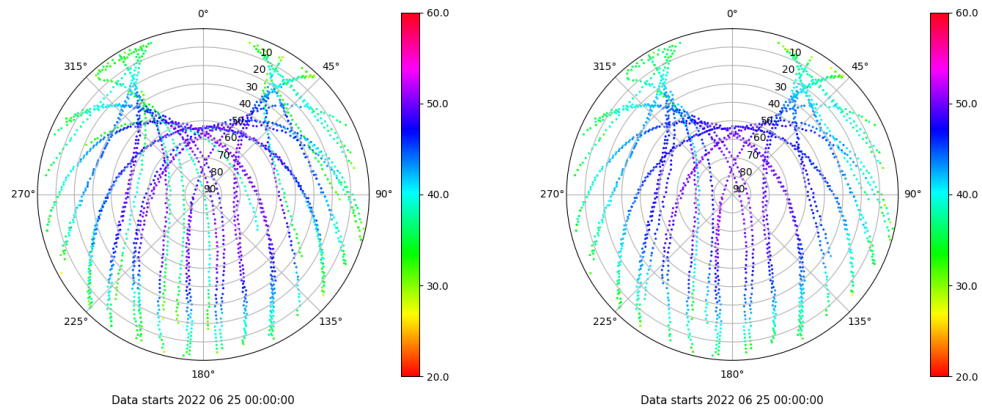
Skyplot for station SEV1. Signal to Noise S1C Data file SEV100ESP_R_2022176.xtr Skyplot for station SEV1. Signal to Noise S2C Data file SEV100ESP_R_2022176.xtr
