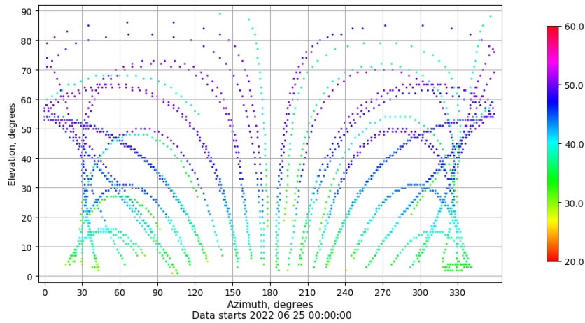
Azimuth-elevation plot for station SEV1. Signal to Noise S1C Data file SEV100ESP_R_2022176.xtr
