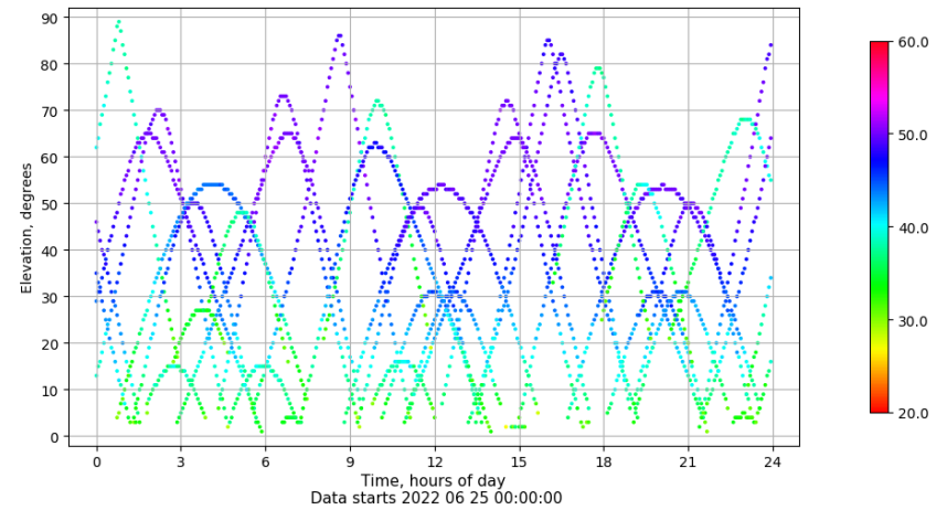
Time-elevation plot for station SEV1. Signal to Noise S1C Data file SEV100ESP_R_2022176.xtr
