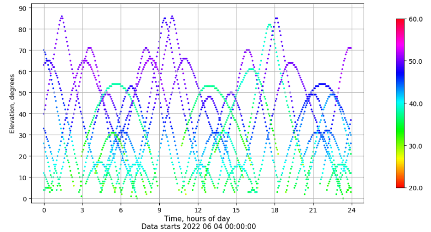
Time-elevation plot for station SEV1. Signal to Noise S1C Data file SEV100ESP_R_2022155.xtr
