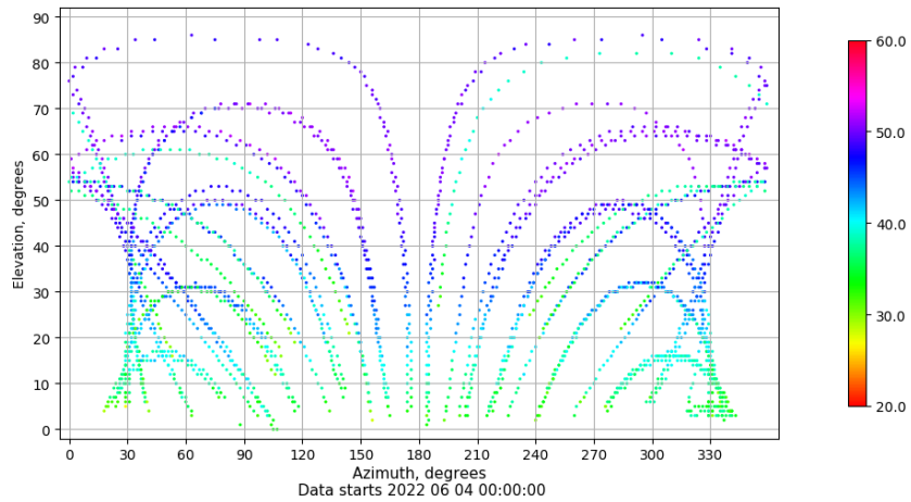
Azimuth-elevation plot for station SEV1. Signal to Noise S1C Data file SEV100ESP_R_2022155.xtr
