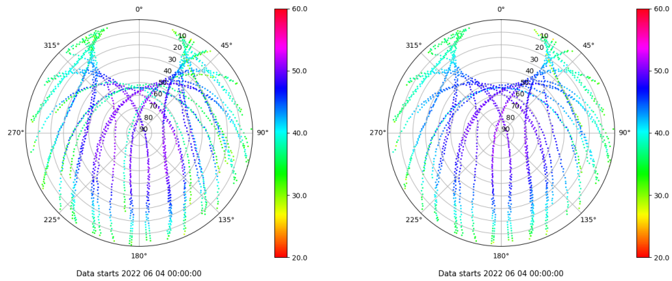
Skyplot for station SEV1. Signal to Noise S1C Data file SEV100ESP_R_2022155.xtr Skyplot for station SEV1. Signal to Noise S2C Data file SEV100ESP_R_2022155.xtr
