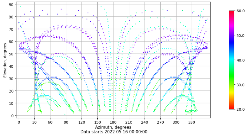
Azimuth-elevation plot for station SEV1. Signal to Noise S1C Data file SEV100ESP_R_2022136.xtr
