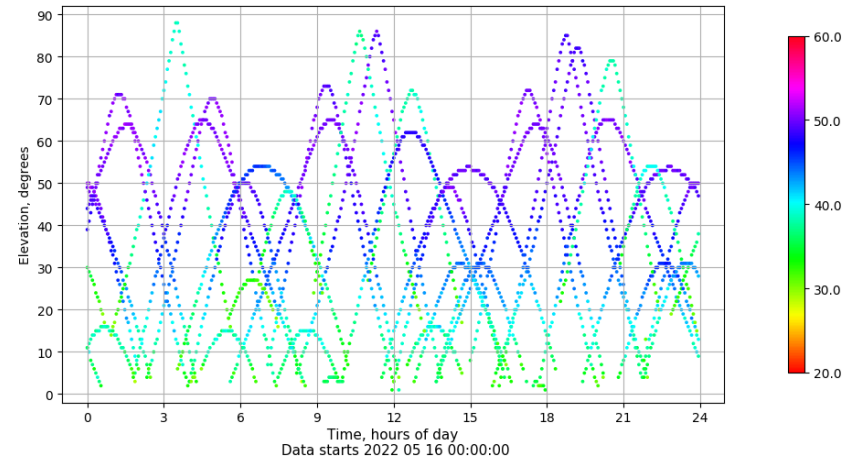
Time-elevation plot for station SEV1. Signal to Noise S1C Data file SEV100ESP_R_2022136.xtr
