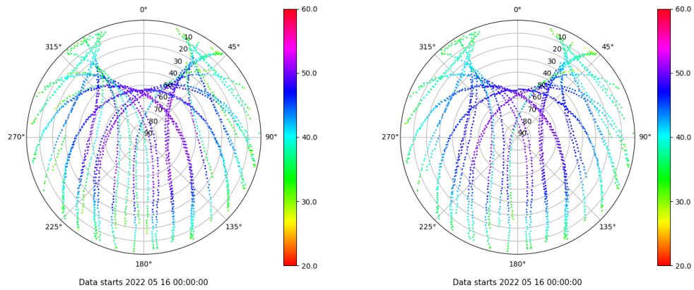
Skyplot for station SEV1. Signal to Noise S1C Data file SEV100ESP_R_2022136.xtr Skyplot for station SEV1. Signal to Noise S2C Data file SEV100ESP_R_2022136.xtr
